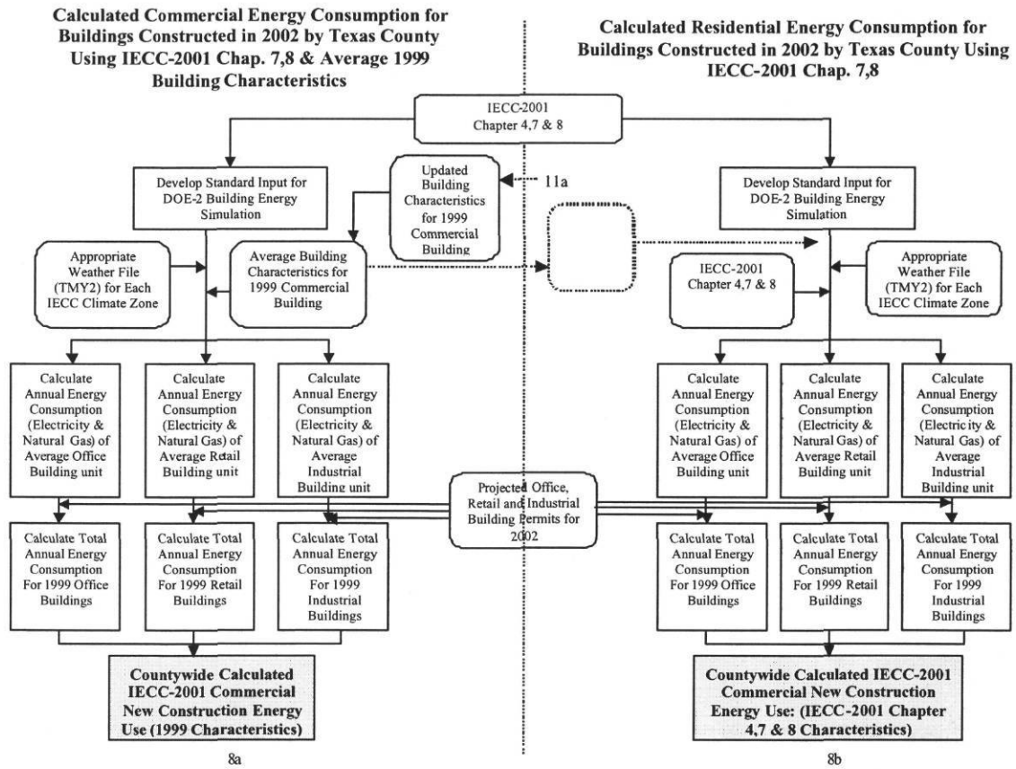
Figure 15: Calculation of countywide commercial new construction energy consumption (1999 characteristics and 2001 IECC/IRC).
