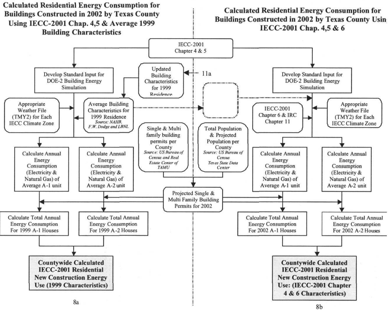
Figure 10: Calculation of countywide residential new construction energy consumption (1999 characteristics and 2001 IECC/IRC).
