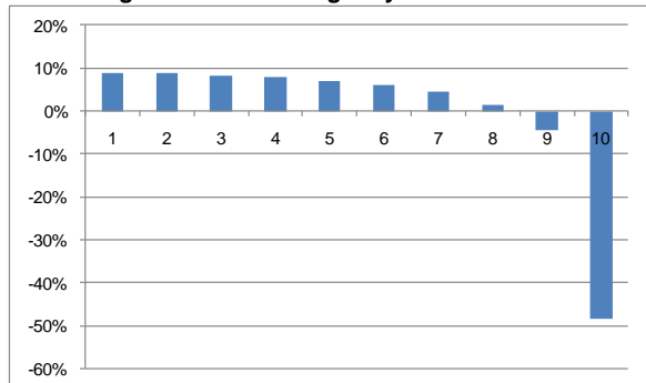
Figure 2E: Mean Weight by Momentum Decile
