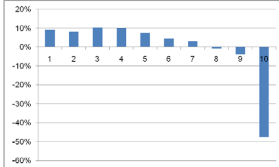
Figure 9E: Mean Weight by Momentum Decile
