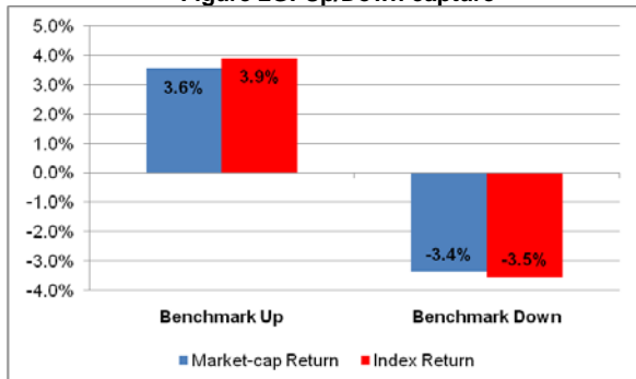
Figure 2G: Up/Down capture
