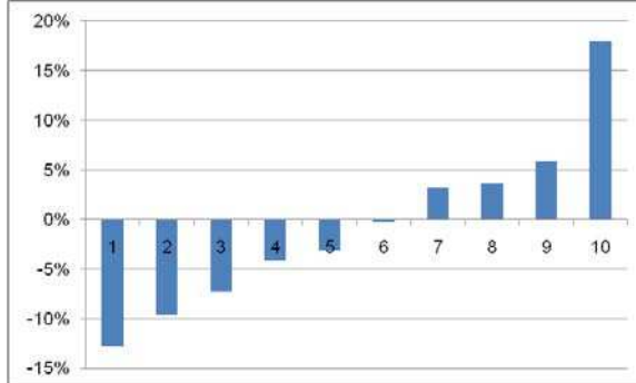
Figure 9F: Mean Weight by Volatility Decile
