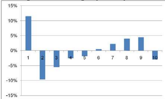
Figure 9G: Mean Weight by Volume Decile
