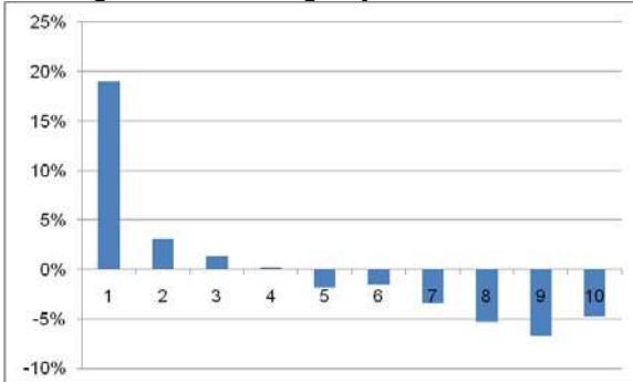
Figure 9G: Up/Down capture
