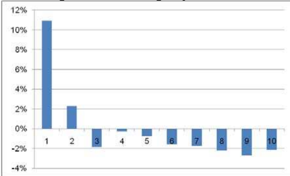
Figure 6D: Mean Weight by BTMV Decile
