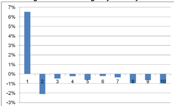
Figure 6H: Mean Weight by Volume Decile
