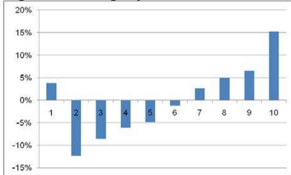
Figure 9I: Mean Weight by semi-deviation Risk Decile
