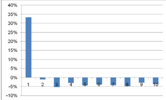
Figure 9D: Mean Weight by BTMV Decile
