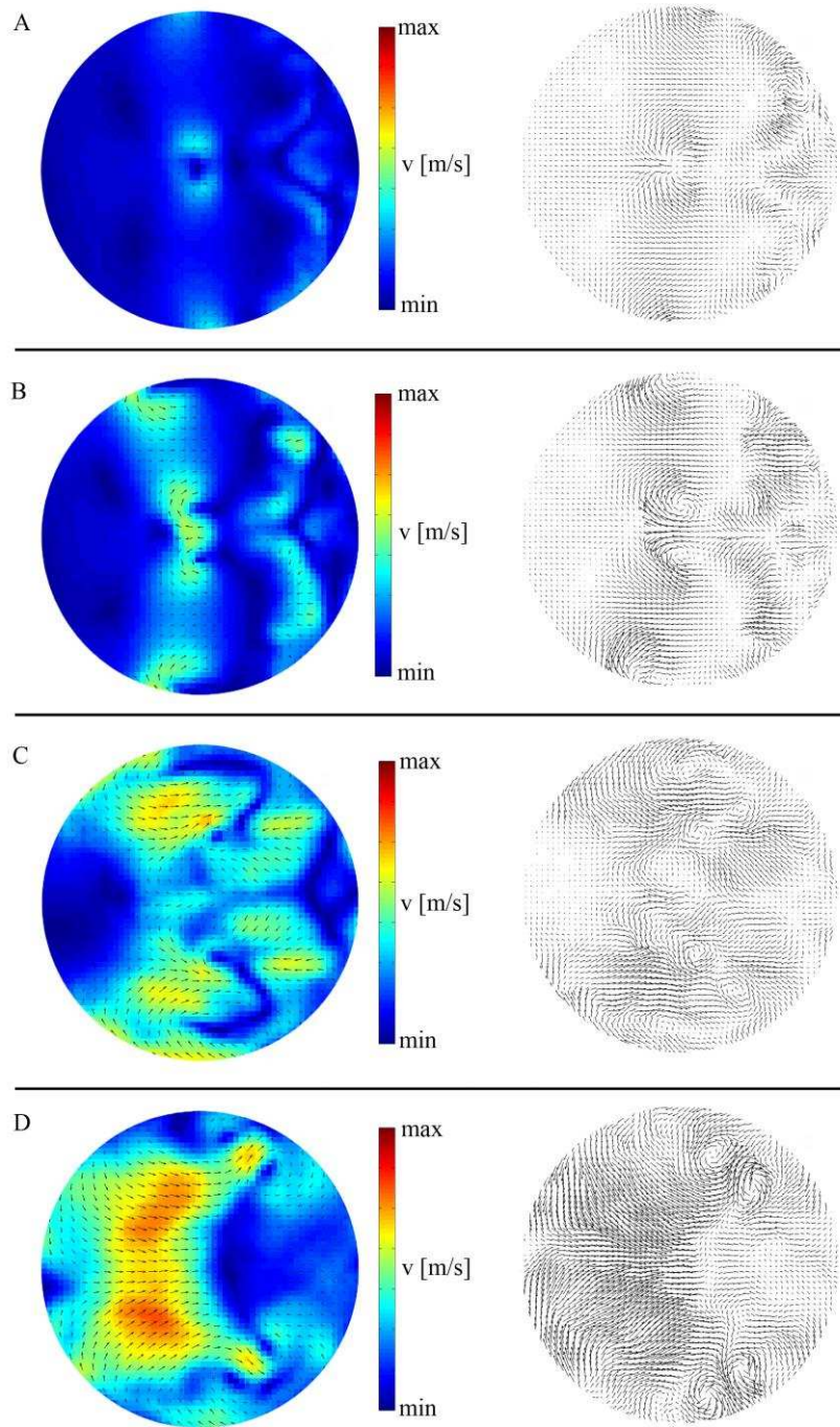
Figure 10. Left: evolution of the phase-averaged velocity field for Crank Angle A, B, C, D, see figure 5 (averaged over 50 cycles, color represents the velocity magnitude); corresponding instantaneous vector fields at the same CA.
