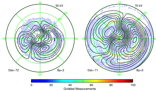
Fig. 8. An illustration of the effect on the SuperDARN convection patterns of including data from the mid-latitude radar on Wallops Island. The shaded areas indicate gridded radar measurements (courtesy, Jo Baker).
