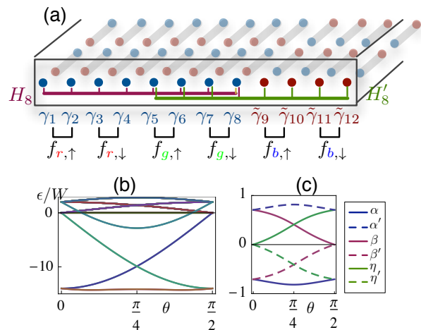
FIG. 1. (color online) (a) Schematic picture of a twelve Majorana chains that interpolate between effective free-fermion classes n = 4 and n = -4 . The interactions terms coupling different Majorana end-states are indicated by thick lines. The ‘‘colored’’ fermions constructed with Majorana fermions are indicated explicitly. (b) Energy spectrum as a function of the interpolation parameter \theta , showing that the spectrum remains gapped through the interpolation. The ground state is two-fold degenerate. (c) Amplitudes \alpha, \alpha', \beta, \beta', \gamma , and \gamma' for the ground state wavefunctions, as a function of the interpolation parameter \theta , see Eq. (9).
