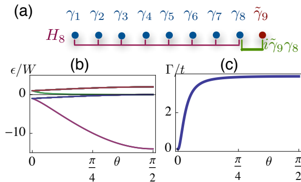
FIG. 2. (a) Schematic picture a nine channel setup that allows for an interpolation between the topologically equivalent effective free-fermion phases with n = 7 and n = -1 . (b) Energy spectrum of the low energy excitations as a function of the interpolation parameter \theta , showing that the system remains gapped throughout the transition. (c) Modulus square of single-particle tunneling matrix elements between the two degenerate ground states, as a function of \theta .
