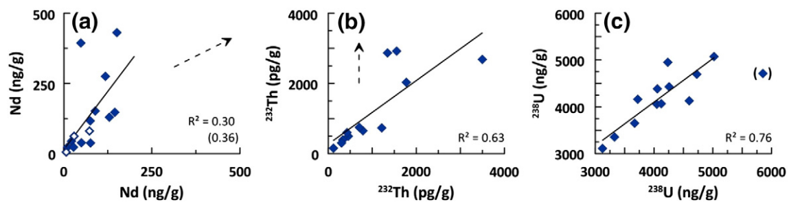
Fig. 9. Trace metal results of different subsamples of the same coral. Dark blue diamonds represent Nd, Th and U data obtained from isotope dilution, i.e., in panel (a) [Nd_{min}] ( <12\% Nd loss), and the white diamonds with blue outline are [Nd_{min}] plotted against accurate Nd concentrations (y-axis) of different subsamples of the same coral (Tables 4 and 6; see text for details). The correlation coefficients were generated by omitting one outlier, which is pointed towards by the dashed arrow in panels (a) (NBP1103 DH74 Gc-2a/b) and (b) (NBP1103 DH43 Dc-8a/b) and displayed in brackets in panel (c). Including the pairs of minimum vs. accurate Nd concentration data in panel (a) increases the linear R^2 to 0.36 (in brackets). For corals NBP1103 DH88 Cc-1 and NBP0805 DR35 Dc-E-1 subsamples 'a' and 'b' were chosen for correlation, respectively.
