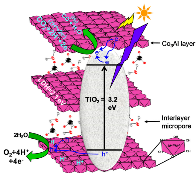
Scheme 2. Proposed mechanism of CO 2 photoreduction due to heterojunction formation within over P25@CoAl-LDH nanocomposite.
