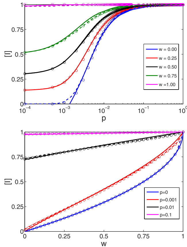
Figure 3. Dependence of the disease prevalence [I]^* on infectiousness p (top) and fraction of infected arrivals w (bottom). The disease prevalence increases monotonically with infectiousness p and fraction of infected arrivals w . In agent-based simulations (circles), [I]^* is calculated over the surviving runs among 10^3 total realizations. Homogeneous approximation (solid lines) is the analytical solution of Eq. (8). Heterogeneous approximation (dashed lines) is the stationary value of the numerical integration of Eq. (3). Parameters: r=q=0.01 , m_0=6 , m=5 .
