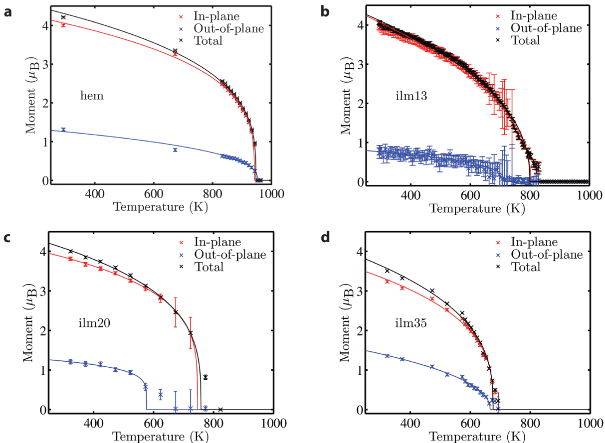
FIGURE 4. Refined in-plane ( M_{\parallel} ), out-of-plane ( M_{\perp} ), and total ( M_{\text{tot}} ) moment as a function of temperature for samples hem, ilm13, ilm20, and ilm35. The solid lines are power law fits. The error bars represent one standard deviation ( \sigma ).
