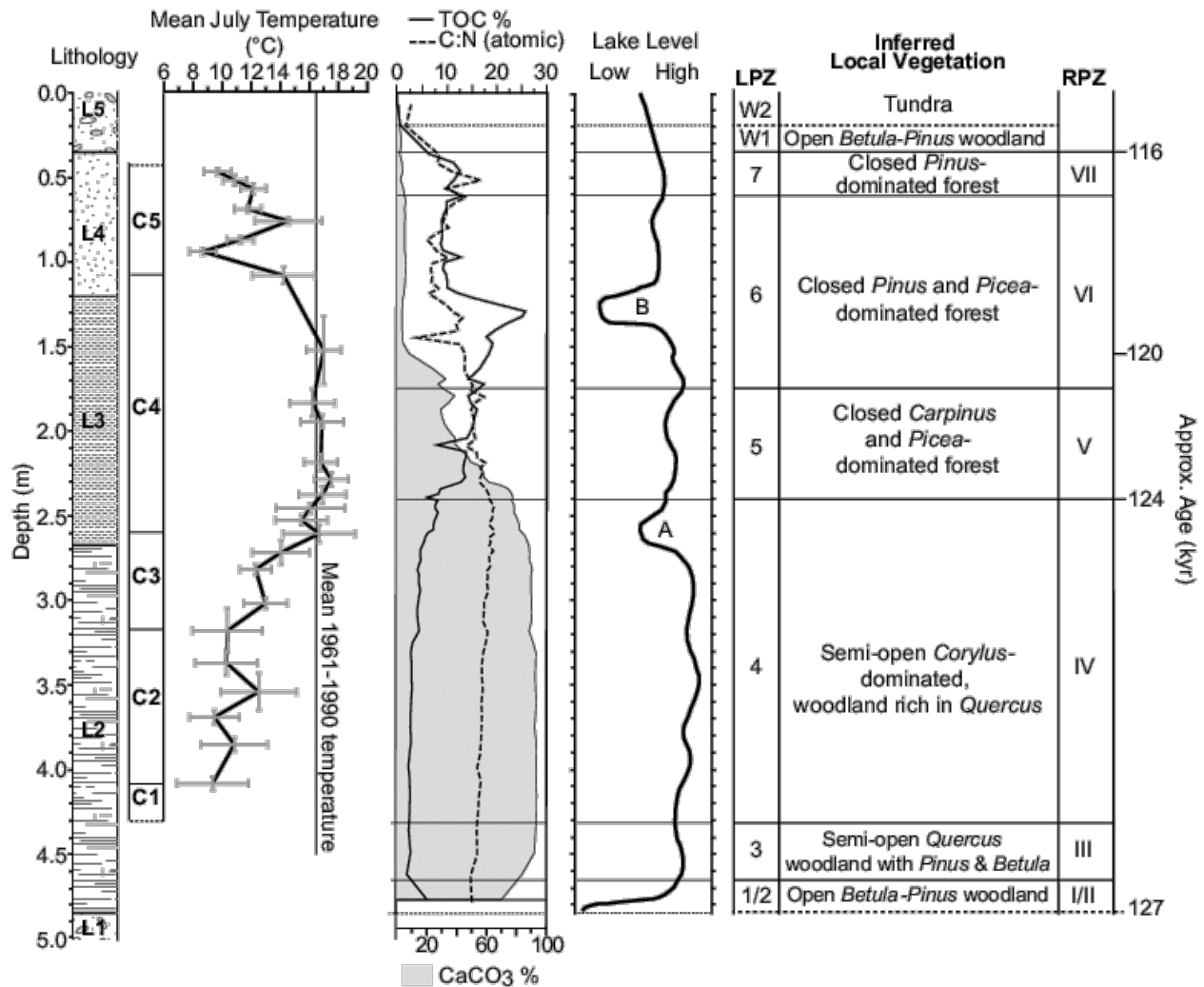
Figure 3. Chironomid-inferred mean July temperature for Hollerup (Denmark) compared against key lithological (percent total organic carbon [TOC], carbon:nitrogen [C:N], percent CaCO 3 ) and lake-level data. Local pollen zone (LPZ) scheme and inferred local vegetation are plotted in relation to regional pollen zone (RPZ) scheme for northern Europe (Grøger, 1991; Møller, 1974) (Table DR1 [see footnote 1]). L1-L5-lithologic units (see Fig. 2); C1-C5-chironomid assemblage zones (see Fig. 2)
