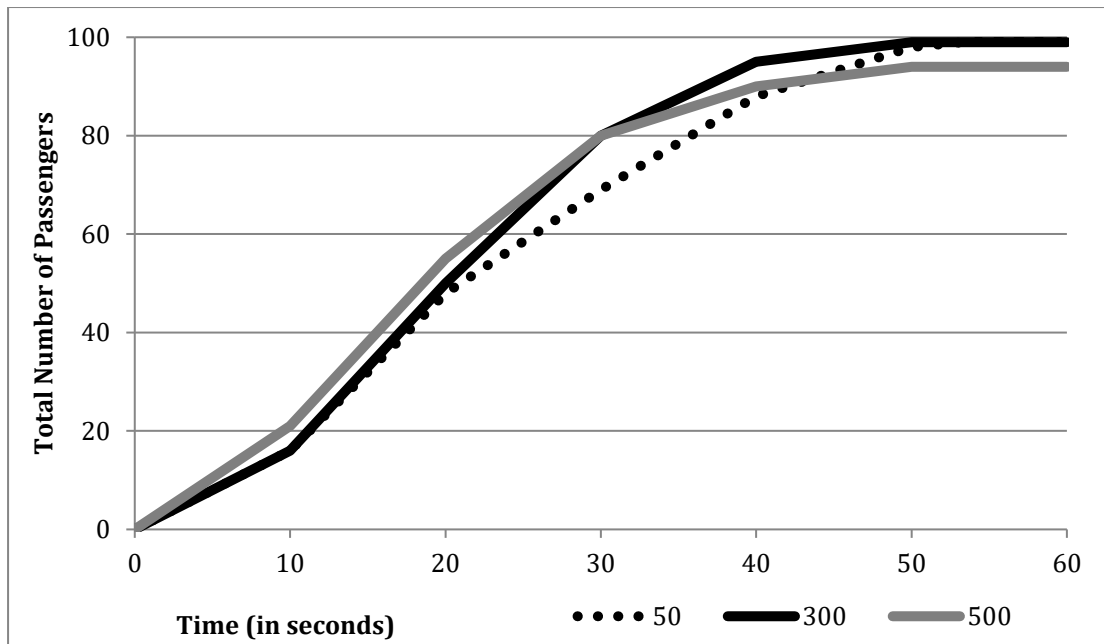
Figure 9: Cumulative number of passenger movements during the door open time for different standback arrangements, majority boarding scenario
