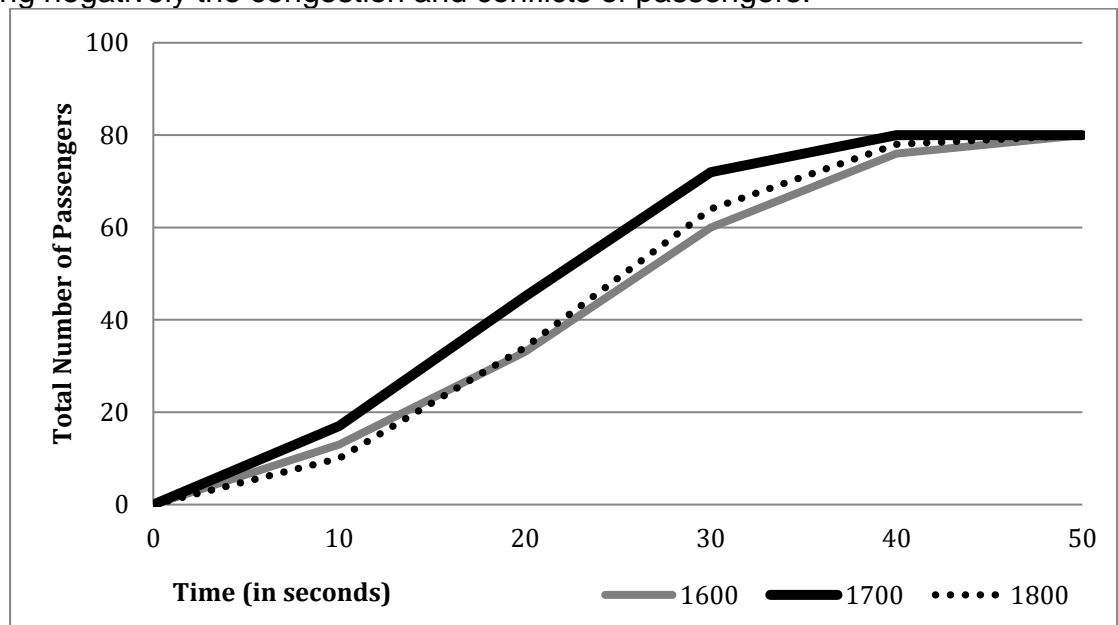
Figure 4: Cumulative number of passengers boarding or alighting throughout door open time.
