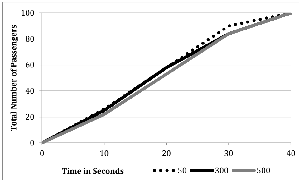
Figure 8: Cumulative number of passenger movements during the door-open time, according to standback, majority alighting scenario
