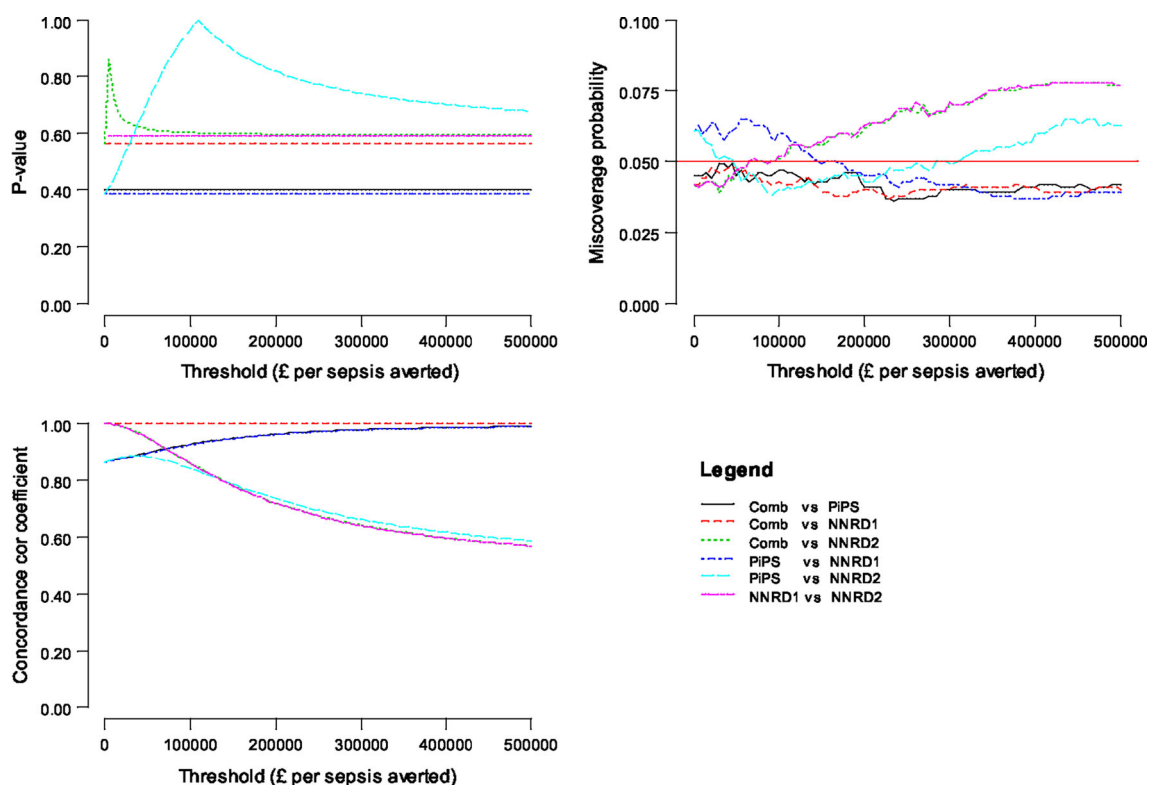
Fig. 3 Two-sided p values, probability estimates of miscoverage and concordance correlation coefficients for comparing the agreement between cost-effectiveness estimates from the PiPS, NNRD, and
