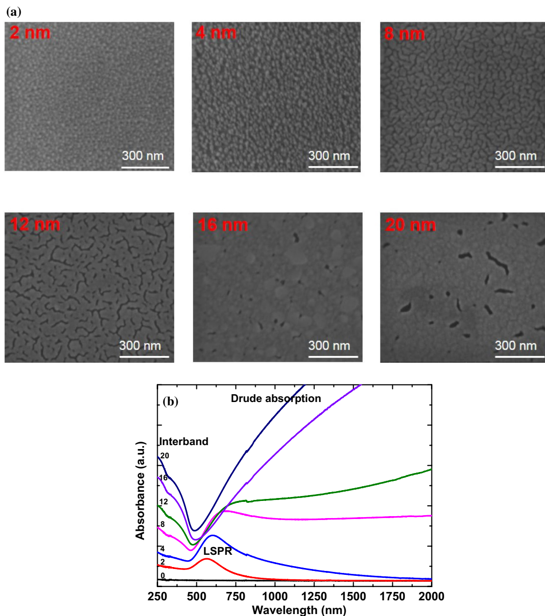
Fig. 1 a High Resolution SEM images of Au thin films (2–20 nm) thermally evaporated on quartz slides (deposition rate of 0.2 Å/s and at a pressure of 1 \times 10^{-6} torr), b UV-Vis-IR absorbance spectra of Au thin films with different thickness (in nm) on quartz slides
