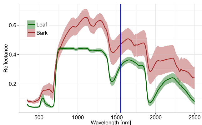
Fig. 6. Leaf and bark spectral reflectances of a deciduous woodland, Wytham Woods, U.K. The solid line indicates the weighted average spectral reflectance and the area around the mean represents the 95% coverage interval. The weights are allocated based on the number of trees per species, with Acer pseudoplatanus (55%), Fraxinus excelsior (20.6%), and Corylus avellana (14.3%) being the dominating species. Data were captured with an ASD spectrometer in the summer of 2015. The vertical blue line represents the wavelength of the RIEGL VZ-400 (1550 nm).
