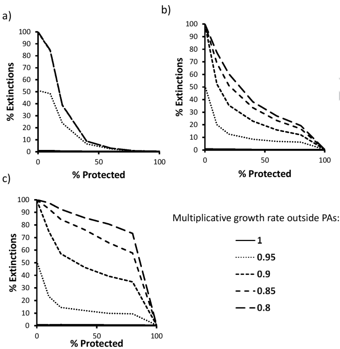
Fig. 2. Scenario modelling of a population of cheetah living on unprotected and protected lands. Starting population is 200 individuals distributed at a varying proportion between protected and unprotected lands (x axis). Multiplicative growth rate ( \lambda ) inside PAs is 1.0 but outside PAs is allowed to vary from this rate down to 0.8. Graphs show estimated extinction rates under three migration scenarios: a) no migration between protected and unprotected lands; b) medium migration rate between protected and unprotected lands of 0.05 and standard deviation 0.025; and c) high migration rate of 0.1 and standard deviation 0.05. Results are reported from 1,000 simulations over 50 years.
