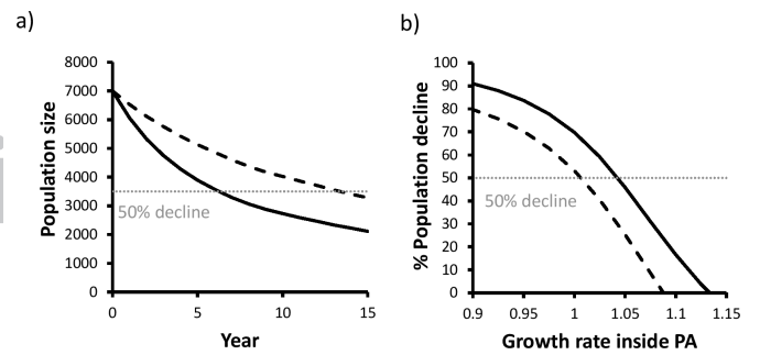
Fig. 3. Simulated a) population trajectories over three generations (15 years) of the global cheetah population and b) sensitivity analysis to changes in the growth rate within PAs. Starting population was the current total estimated global population size of 7,000 individuals with 33% of the population on protected lands (Table 1). The dashed line depicts results from a multiplicative growth rate ( \lambda ) of 0.9 on unprotected lands, the solid line 0.8. Migration rate was set at 0.05 with standard deviation 0.025. Results are reported from 1,000 simulations and all other parameters of the model are as described for Fig. 2. The grey dotted line depicts the 50% threshold for up-listing to Endangered status using IUCN Red List criteria A3b (a population size reduction of \geq 50\% , projected or suspected to be met within the next three generations, based on an index of abundance (28)).
