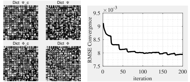
(a) Learned coupled HR dictionaries (b) Training error convergence
