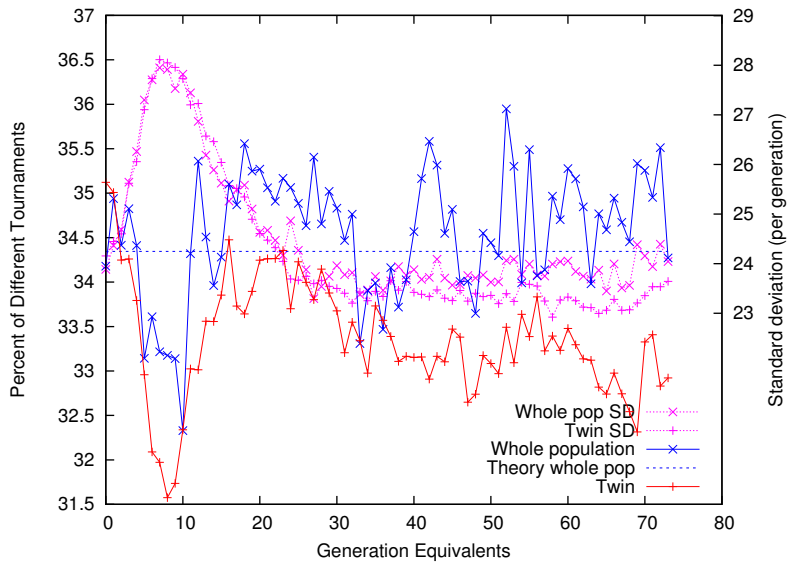
Fig. 6. Evolution of expected fraction of binary tournaments with different outcome in typical kin selection run with population of 10 000 (+). (Same run as Figure 4.) Expected fraction for whole population plotted \times for comparison. Twin's fitness gives same outcome slightly more often than using the population.
