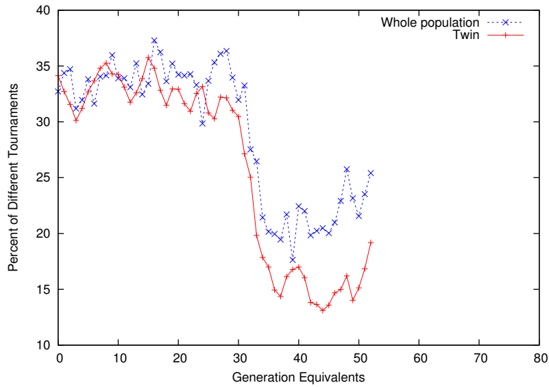
Fig. 5. Evolution of expected fraction of binary tournaments with different outcome in typical twin run with population of 1000 (+). (Same run as Figure 1.) Expected fraction for whole population plotted \times for comparison. Ties are broken at random.
