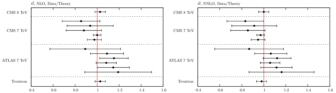
Figure 4: The MMHT fit to \sigma_{t\bar{t}} data, figures from [6].
