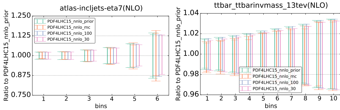
Figure 13: Examples of differential cross sections using each means of combination, figures from [15].
