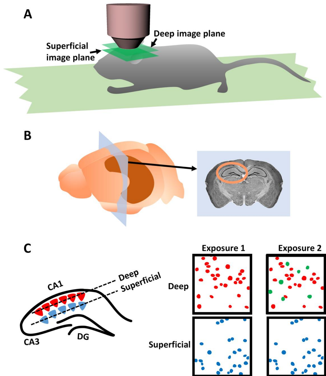
Figure 1. Differential stability of place cells in deep and superficial layers of the hippocampal CA1 subfield. (A) A mouse transfected with a viral calcium imaging protein (GcAMP6f) in dorsal hippocampus ran on a treadmill while its CA1 neurons were imaged in two planes, deep and superficial, by an overhead two-photon microscope. (B) Schematic of the mouse brain and hippocampus. The coronal section on the right represents the plane indicated in blue on the left; the region of the dorsal hippocampus is circled. (C) Imaging of deep and superficial CA1 neurons. Left – schematic of the dorsal hippocampus showing the pyramidal neurons in CA1, and the imaging planes. Right – schematic of active neurons as
