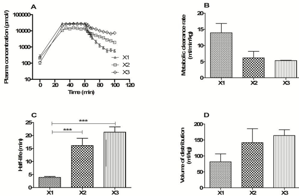
Figure 3: Plasma concentrations of peptides X1, X2 and X3, and their pharmacokinetic parameters (metabolic clearance rate, half-life and volume of distribution) using the surgical rat model in anesthetised male Wistar rats. A: Semi-logarithmic plasma concentration of peptides over time, B: Metabolic clearance rate of peptides, C: Half-life of peptides and D: Volume of distribution of peptides. For all experiments n=4. Statistics with one-way ANOVA. ***=p<0.001.
