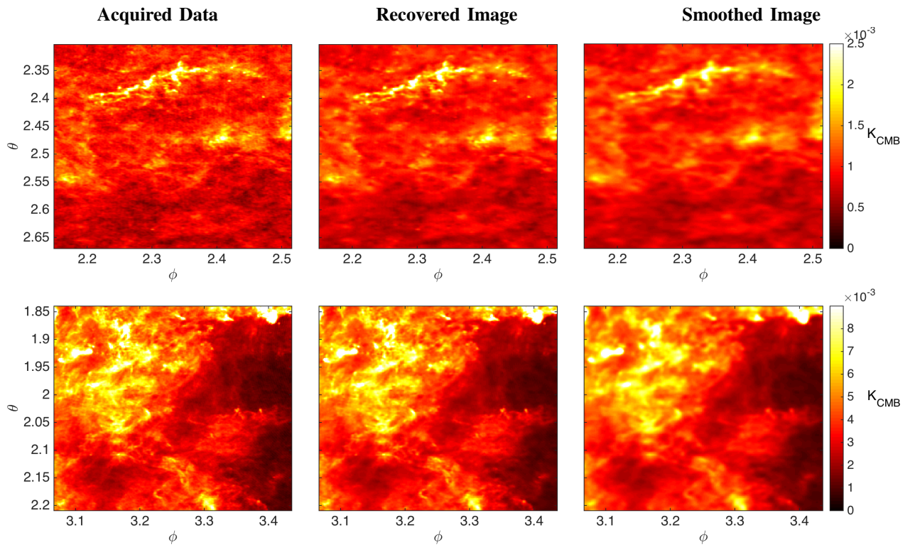
Fig. 6. Results from denoising the Planck 353 GHz total intensity map. The left column shows the acquired data, the middle column shows the denoised data and the right column shows the data denoised by smoothing with a 5 arcmin Gaussian kernel (the standard approach [69]). Each plot shows a zoomed region of the sphere. The acquired data shown here is a zoom in of that shown in Fig. 5, the top figure is the blue region and the bottom figure is the green region.
