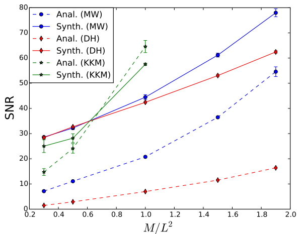
Fig. 3. Reconstruction performance averaged over 10 realisations for the DH (red diamonds), MW (blue circles) and KKM (green stars) sampling schemes, when solving the low resolution inpainting problem in the analysis setting (dashed lines) and the synthesis setting (solid lines). The KKM and MW sampling schemes provide enhancements in reconstruction quality when compared to the DH sampling scheme. The synthesis setting is shown to be generally superior to the analysis setting.
