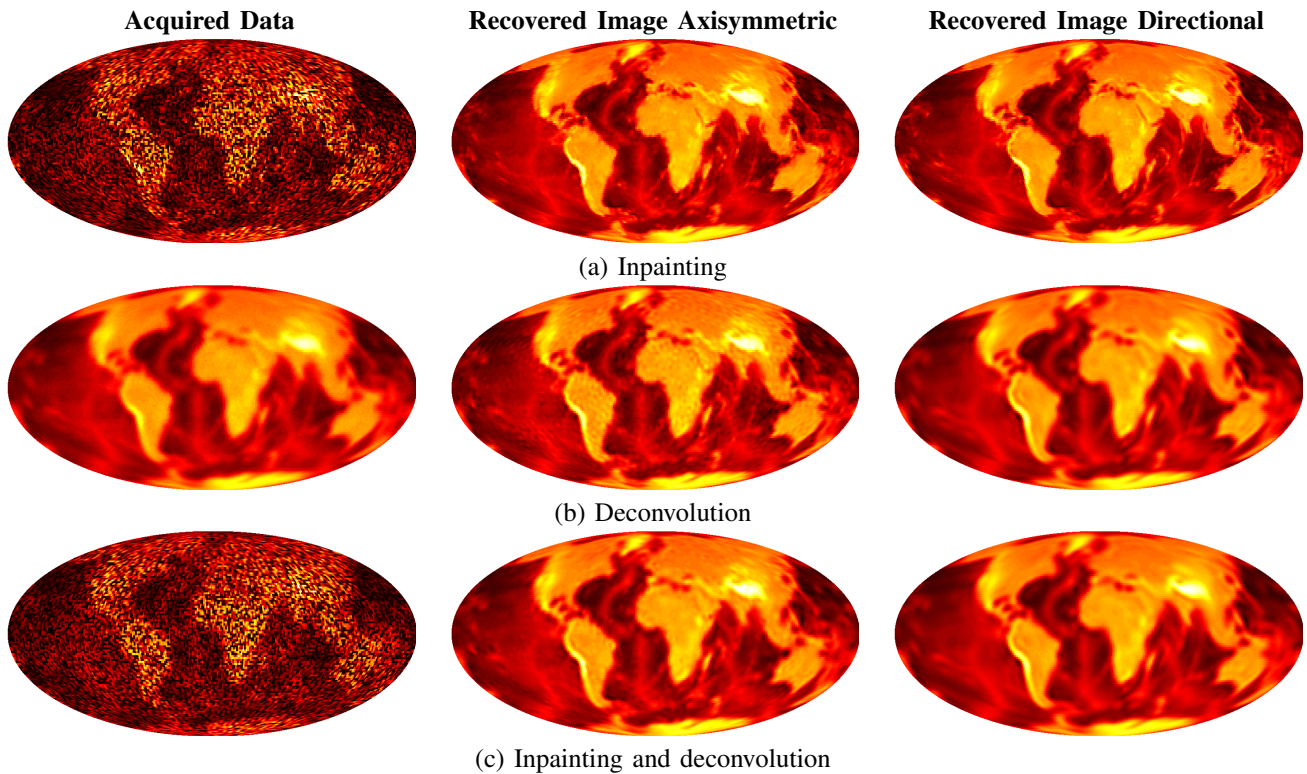
Fig. 4. Reconstructed images from the high resolution experiments described in Sec. IV-B. All problems are solved in the synthesis setting using MW sampling. Each solution is presented next to a band limited representation of the measured data. The SNR of the reconstructions are (a) 57.1 dB, (b) 51.8 dB and (c) 50.8 dB for the axisymmetric wavelets and (a) 58.4 dB, (b) 48.5 dB and (c) 48.5 dB for the directional wavelets. For the inpainting problem directional wavelets yield superior performance, while for the deconvolution and joint inpainting and deconvolution problems the SNR recovered with axisymmetric wavelets is superior, albeit visual artefacts are mitigated when using directional wavelets.
