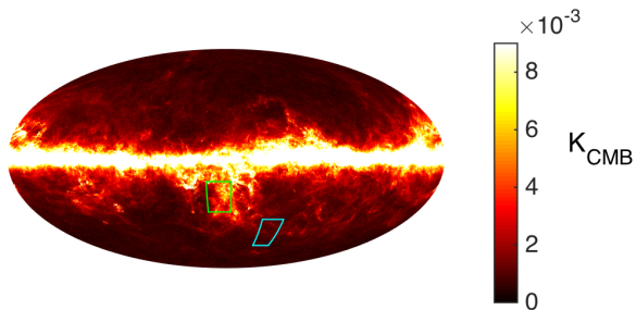
Fig. 5. Acquired data of the 353 GHz Planck total intensity map. A full description of how this data was acquired can be found in Sec. V. The regions highlighted are shown in more detail in Figure 6.
