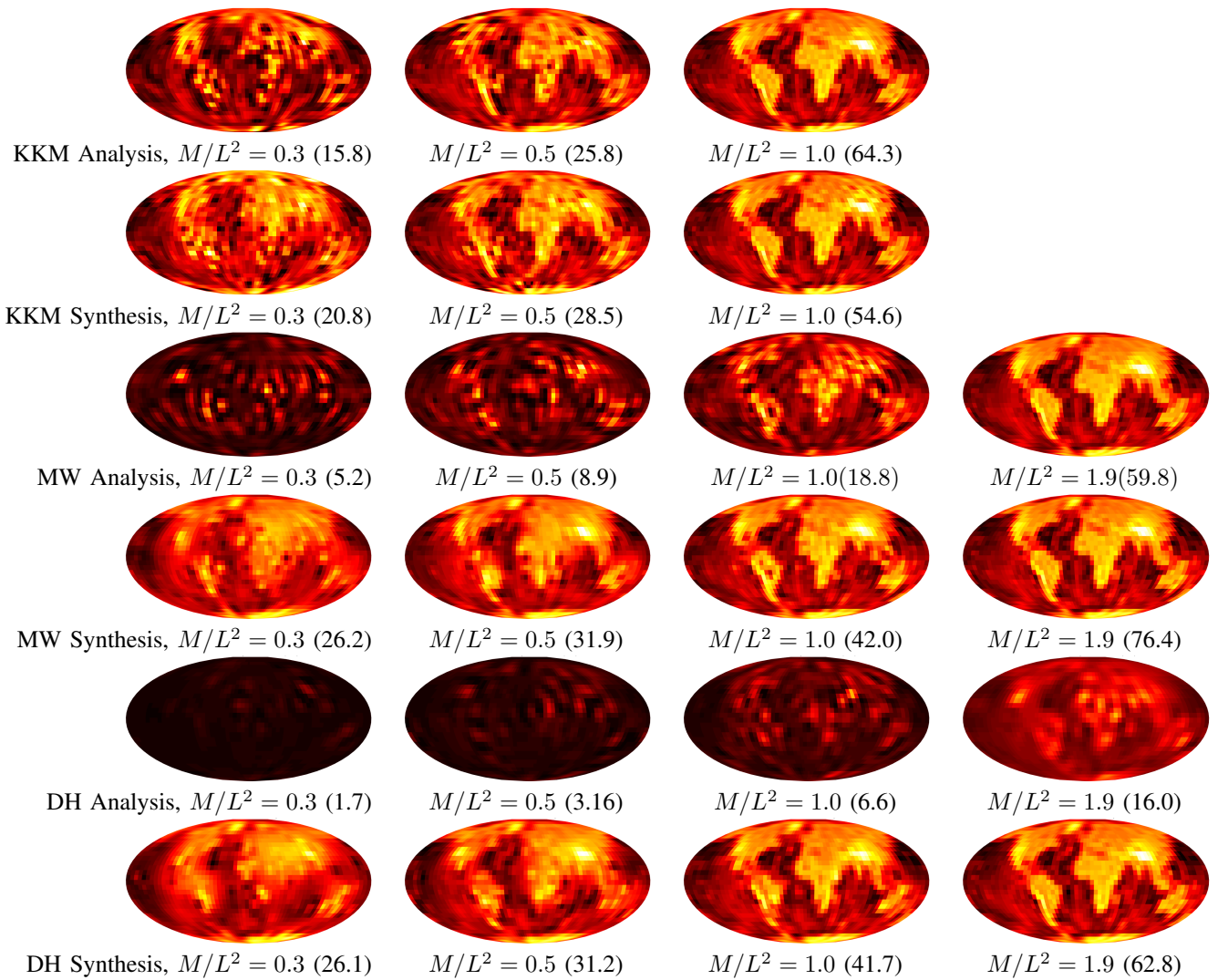
Fig. 2. Reconstructed images from the low resolution inpainting experiment described in Sec. IV-A. The first two rows show the reconstruction using KKM sampling when solving the analysis and synthesis problems, respectively. The third and fourth rows are solutions to the same problems with MW sampling, and fifth and sixth rows correspond to DH sampling. Each column corresponds to a different number of measurements. The SNR for each image is giving in brackets in dB. The synthesis setting generally out-performs the analysis setting, while sampling schemes that require fewer samples generally out perform those requiring more samples.
