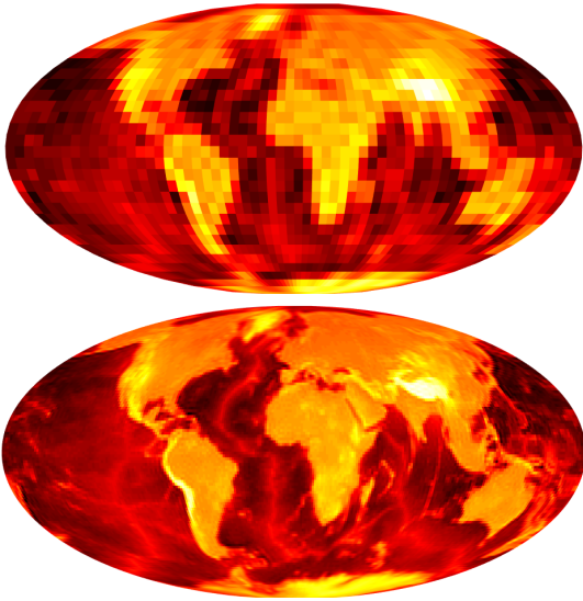
Fig. 1. Test images of Earth topographic data constructed to be band-limited at L = 32 (top) and L = 128 (bottom). These images constitute the ground truth in our numerical experiments. Here and subsequently data on the sphere are displayed using the Mollweide projection, with zero values shown in black, unit values shown in yellow, and the colour of intermediate values interpolated between these extremes.
