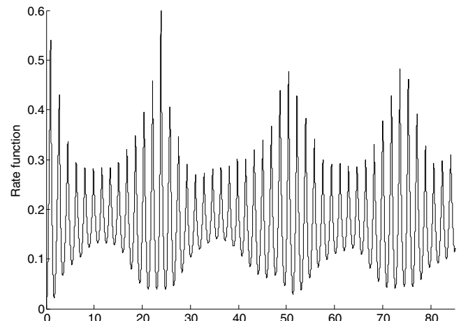
FIG. 12. The rate function vs time in the z basis for six-site uCPS overlap compared with the exact evolution. The quench corresponds to the ground state of the quantum Ising Hamiltonian with h = 1.5 (paramagnetic phase) evolved with the h = 0.1 Hamiltonian (ferromagnetic phase).
