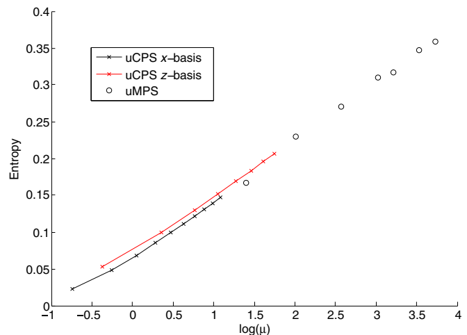
FIG. 10. The scaling of uCPS/uMPS entanglement entropy S vs \ln(\mu) , where \mu is the correlation length. The slope approaches a constant value, which is theoretically predicted to be \frac{c}{6} , where c is the central charge.
