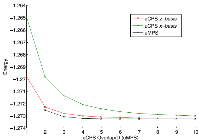
FIG. 4. Convergence of uCPS and uMPS ground-state energies for the transverse Quantum Ising model at the criticality. The x axis denotes an overlap size for uCPS data and a bond dimension for uMPS data.
