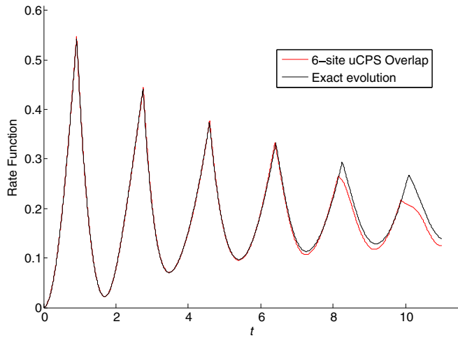
FIG. 12. The rate function vs time in the z basis for six-site uCPS overlap compared with the exact evolution. The quench corresponds to the ground state of the quantum Ising Hamiltonian with h = 1.5 (paramagnetic phase) evolved with the h = 0.1 Hamiltonian (ferromagnetic phase).
