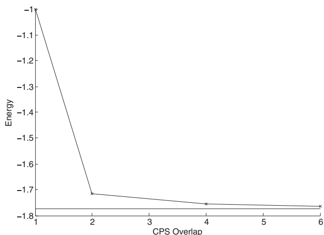
FIG. 6. Convergence of uCPS ground-state energies for the Heisenberg model. The horizontal line denotes the exact energy. Whilst the uCPS approximations are not basis dependent, convergence turns out to be very slow.
