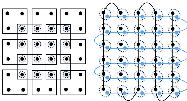
FIG. 1. The diagram on the left-hand side depicts a CPS in two dimensions with single-site overlaps. The squares represent the C tensors, and the black dots denote the spins, each C tensor thus having four indices. The right-hand side depicts a string bond state consisting of a product of two matrix product states, each covering the entire lattice. The dashed circles are present at sites where the underlying CPS/string bond state tensors overlap, and each such circle can be understood as representing the copier tensor projecting the indices in the overlap onto the physical spin.
