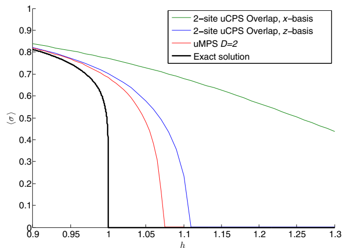
FIG. 11. Both uCPS and uMPS are capable of capturing the quantum Ising model equilibrium phase transition, from the ferromagnetic phase, h < 1 , characterized by a nonzero value for the order parameter operator expectation value \langle \sigma^z \rangle , to the paramagnetic phase h > 1 when \langle \sigma^z \rangle = 0 . The accuracy of the uCPS approximation for the critical point, h = 1 , degrades as a function of the rotation angle away from the z basis. In the x basis, the phase transition is entirely missed.
