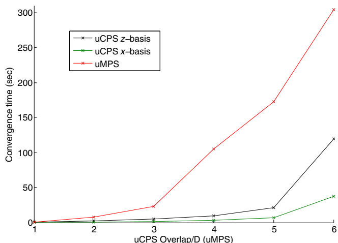
FIG. 5. Convergence times for uCPS and uMPS approximations for the ground state of the quantum Ising model at criticality. The x axis denotes an overlap size for uCPS data and a bond dimension for uMPS data.
