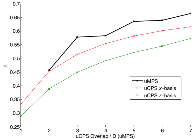
FIG. 8. Correlation length \mu as a function of uCPS overlap/uMPS bond dimension D , for the quantum Ising model in the ordered gapped phase ( J = 1 and h = 0.5 ).
