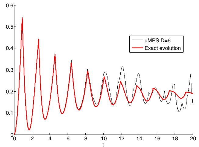
FIG. 14. Rate function vs time in z basis exhibits recurrence when projected to the uCPS manifold. Recurrence is exact for one-site CPS overlap (top), and approximate when the overlap is larger than one, as demonstrated for the three-site uCPS overlap case (middle). The uMPS approximation does not exhibit recurrences at large times; beyond the point at which the rate function is accurately captured, the behavior is chaotic (bottom), and the precise behavior is also highly bond-dimension dependent.
