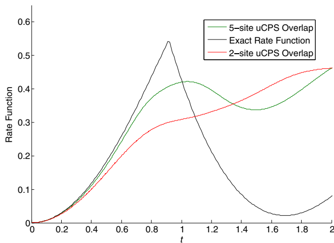
FIG. 13. The uCPS approximation, for two- and five-site uCPS overlap in the x basis, of the rate function for the h = 1.5 \rightarrow h = 0.1 quench in the quantum Ising model. In this basis uCPS completely misses the dynamical phase transition. The behavior of the uCPS approximation is analytical even at large times (not displayed).
