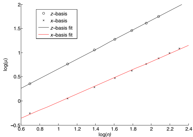
FIG. 9. The logarithm of the correlation length \mu vs the logarithm of uCPS overlap for uCPS ground-state approximations for the quantum Ising model at criticality, for both the x - and z -basis choices. In the z basis, the linear fit is particularly accurate, with slope equal to one to good approximation.
