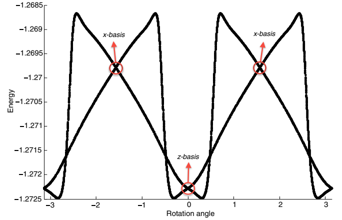
FIG. 3. The behavior of two-site overlap uCPS ground-state energy approximations for the quantum Ising model at criticality, as a function of the global rotation angle around the y axis away from the z -basis choice. The TDVP algorithm exhibits unique convergence to the global minimum only at the points marked by the red circles, which denote the z - and x -basis choices, and at one intermediate point. In general, depending upon the details of the initial random state, imaginary-time TDVP will converge to one of the minima associated with the splitting of otherwise degenerate energy levels, which occurs due to the lack of rotation invariance of the uCPS Ansatz .
