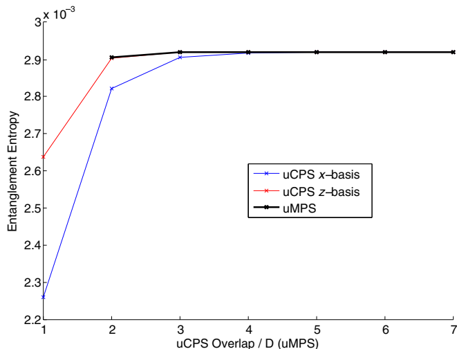
FIG. 7. Entanglement entropy S as function of uCPS overlap/uMPS bond dimension D , for the quantum Ising model in the ordered gapped phase ( J = 1 and h = 0.5 ).
