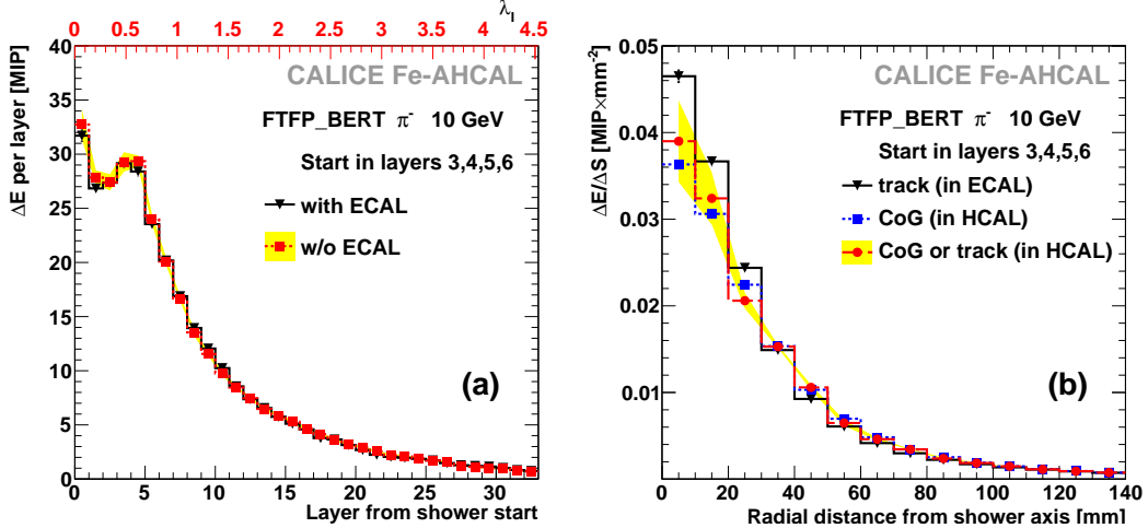
Figure 18. Shower profiles of simulated 10 GeV negative pions which start showering in physical layers 3,4,5 or 6 of the AHCAL: (a) longitudinal profiles obtained with (black triangles) and without (red circles) ECAL, (b) radial profiles with respect to shower axis estimated from track in ECAL (black triangles), shower centre of gravity (blue squares) and combined method (red circles). The yellow band shows the systematic uncertainty, see appendix A.1 and A.3 for details.
