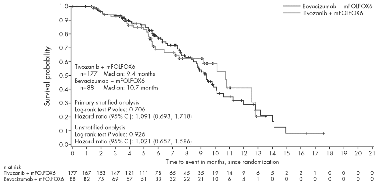
Figure 1: Survival probability of PFS
