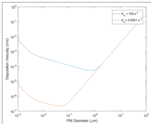
Figure 1. Relationship between particle diameter and deposition velocity calculated with the Crump and Seinfeld model (Nazaroff et al. 1994)
