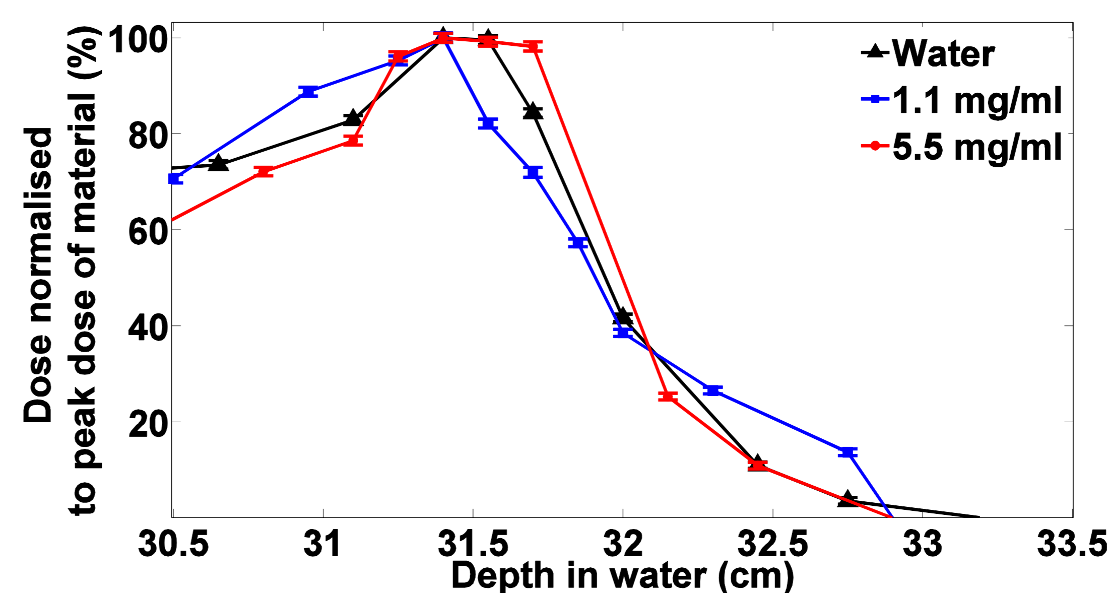
Figure 4: Depth dose plot normalized to peak dose of the material to show the changes caused to the shape of the Bragg peak with GNP concentrations of 1.1 and 5.5 mg/ml. Errors correspond to two standard deviations.
