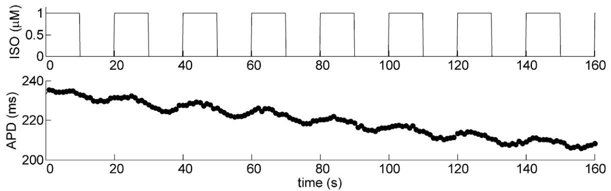
Figure 2. Protocol of phasic isoproterenol (ISO) application (top panel) and corresponding time course of action potential duration (APD) changes (bottom panel) computed using the O'Hara-Xie-modNiederer model.
