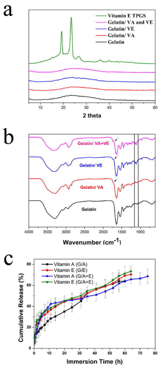
Figure 3. a) XRD patterns of vitamin E TPGS and the cross-linked nanofibers prepared in this work; b) FTIR spectra of the cross-linked fibers; c) the in vitro release profiles of vitamins from G/A, G/E and G/A+E fibers
