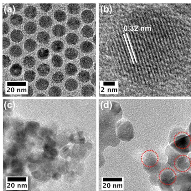
Figure 2. High resolution TEM for CuInS 2 /ZnS NCs and NiO photocathodes. (a) CuInS 2 /ZnS NCs HRTEM. (b) Lattice fringes of CuInS 2 /ZnS NCs shown to be 0.32 nm. (c) NiO photocathode film without NCs. (d) NiO photocathode film with NCs.
