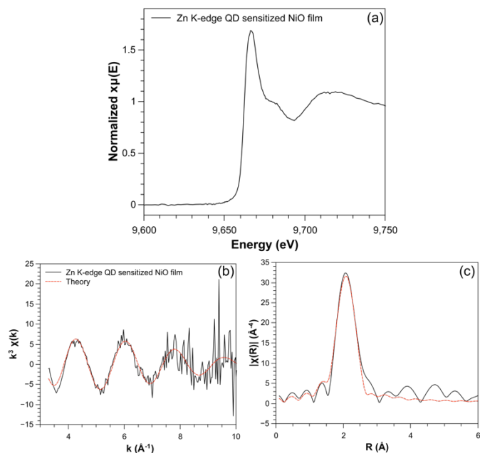
Figure 5. Zinc K-edge (a) XANES, (b) EXAFS and (c) Fourier transform of NC sensitized NiO (black). The solid lines (black) represent experimental data and dashed lines (red) denotes the theoretical model.
