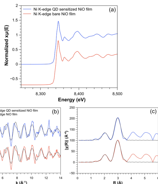
Figure 4. Nickel K-edge (a) XANES, (b) EXAFS and (c) Fourier transform of NC sensitised NiO (blue) and unsensitised NiO (red). The solid lines represent experimental data and dashed lines denote the theoretical model.
