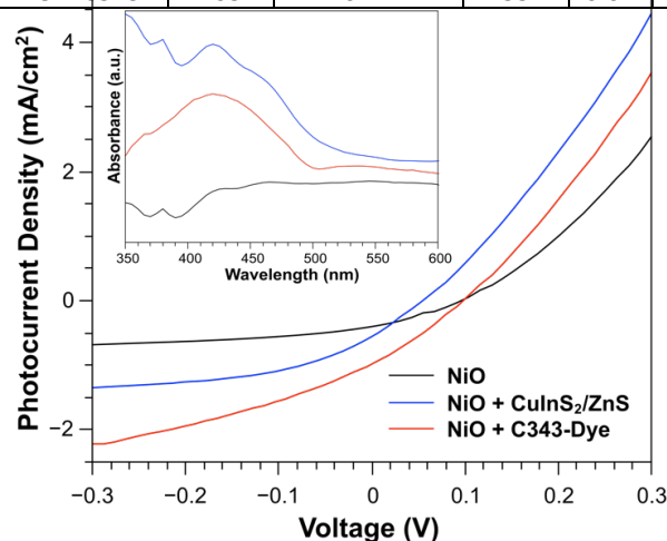
Figure 6. Light JV -Curves for NiO Photocathodes (unsensitised), sensitised with CuInS 2 /ZnS NCs and C343-dye. The illuminated cell area was 0.45 cm 2 . The inset shows the diffuse reflectance absorbance spectra for the corresponding photocathode films.
