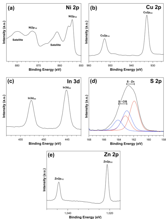
Figure 3. High resolution XPS for CuInS 2 /ZnS on NiO photocathodes. The spectra represent Ni 2p (a), Cu 2p (b), In 3d (c), S 2p (d) and Zn 2p (e).
