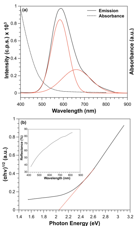
Figure 1. (a) Emission and absorbance spectrum for aqueous CuInS 2 /ZnS quantum dots. The red line indicates the Gaussian fit for emission curve. (b) Tauc absorption plot for band gap estimation. Inset represents the reflectance spectrum for CuInS 2 /ZnS further verifying band gap estimation.
