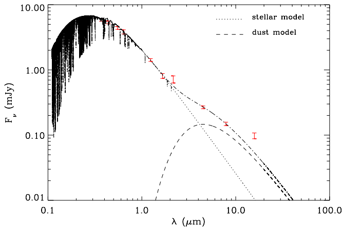
Figure 1. Ultraviolet through infrared energy distribution of GD 61 with photometry represented as error bars. Fluxes below 2 \mu\text{m} (the 2MASS K_s -band measure appears inaccurate and has been ignored) are fitted with a model atmosphere, yielding a photometric distance of 50.1 pc. The dashed line is a flat disk model with inner and outer temperatures of 1300 and 1000 K at i = 79^\circ . The IRS blue peak-up flux is likely to contain significant silicate emission. (A color version of this figure is available in the online journal.)
