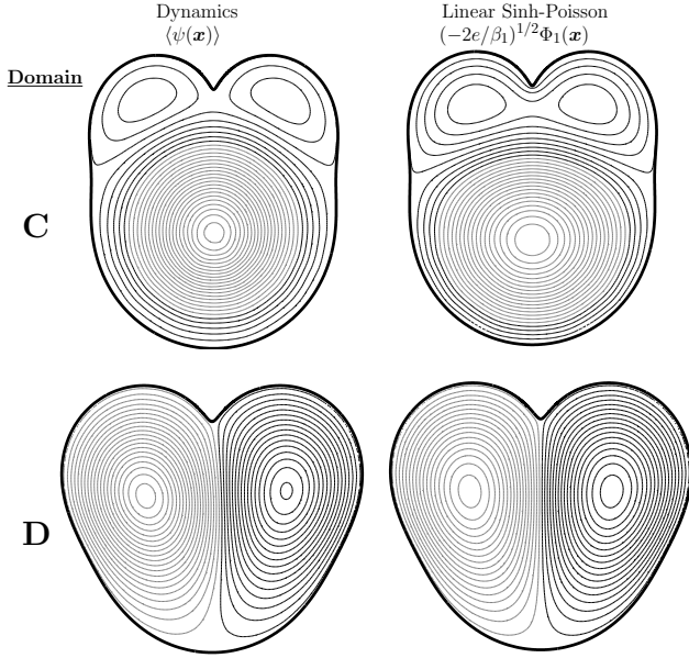
FIGURE 8. Left panels: Time-mean streamfunction (scaled by N\Gamma_0 as in §3.5) \langle\psi(\mathbf{x})\rangle , calculated for time interval 1000\Gamma_0^{-1} < t < 3000\Gamma_0^{-1} , for dynamical runs with N = 100 vortices in domains C and D. The energies are (C) e = E/N^2\Gamma_0^2 = 0.013 ( \varepsilon = 1.3 ) and (D) e = 0.011 ( \varepsilon = 1.1 ). Right panels: Linearised sinh-Poisson solution (-2e/\beta_1)^{1/2}\Phi_1(\mathbf{x}) for the two domains. Contour intervals are the same in each panel.
