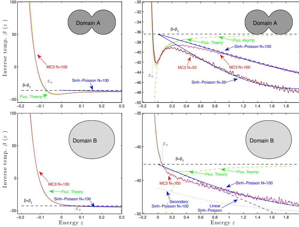
FIGURE 3. Comparison of inverse temperatures \beta_{\mathbf{r}}(E) obtained from the MC3 calculation (red curves) for domains A and B (illustrated), with the theoretical result \beta(\varepsilon) obtained from (3.13) (green curves), and \beta_h(\varepsilon) (see §3.3) obtained from the mean-field (sinh-Poisson) theory (solid blue curves). Left panels are scaled to show the central region and right panels the right-tail region of W(\varepsilon) . The dashed blue lines give the linearised (low E ) sinh-Poisson result and the dashed green lines the large \varepsilon asymptotic result (3.20). A secondary sinh-Poisson solution (dotted blue curve) is shown for domain B.
