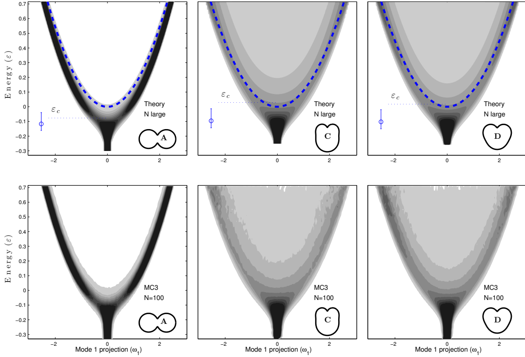
FIGURE 4. Upper panels: Contour plots of p_\varepsilon(\omega_1) , from the theoretical expression (3.15), as a function of (\omega_1, \varepsilon) for domains A, C and D. The blue circle and error bars denote the mean and 95% confidence intervals of W(\varepsilon) and the critical energy \varepsilon_c is marked with a dotted line. The possible values of \omega_1 according to the linearised sinh-Poisson solution (3.28) are marked with the dashed blue parabolas. Lower panels: As for the upper panels, but here p_\varepsilon(\omega_1) is estimated using MC3 sampling of phase-space with N = 100 vortices.
