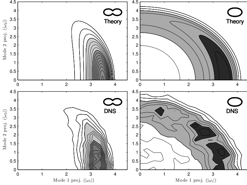
FIGURE 6. Contour plots comparing p_\varepsilon(|\omega_1|, |\omega_2|) (upper panels) predicted by the theory (eqn. 3.16) with (lower panels) statistics compiled from the DNS of eqn. (2.1). The energy is fixed at \varepsilon = 0.05 . Left panels: Domain A. Right panels: Domain B.
