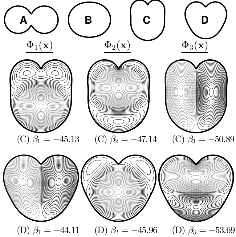
FIGURE 2. Top Row: Domains A-D. Middle Row: Leading three eigenfunctions of domain C. Bottom row: Leading three eigenfunctions of domain D.
