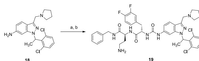
Scheme 7 Reagents and conditions: a) triphosgene, DMAP, THF, 2 , 0-20 °C, 2 h; b) HCl (4 M) in 1,4 dioxane, 20 °C, 2 h
