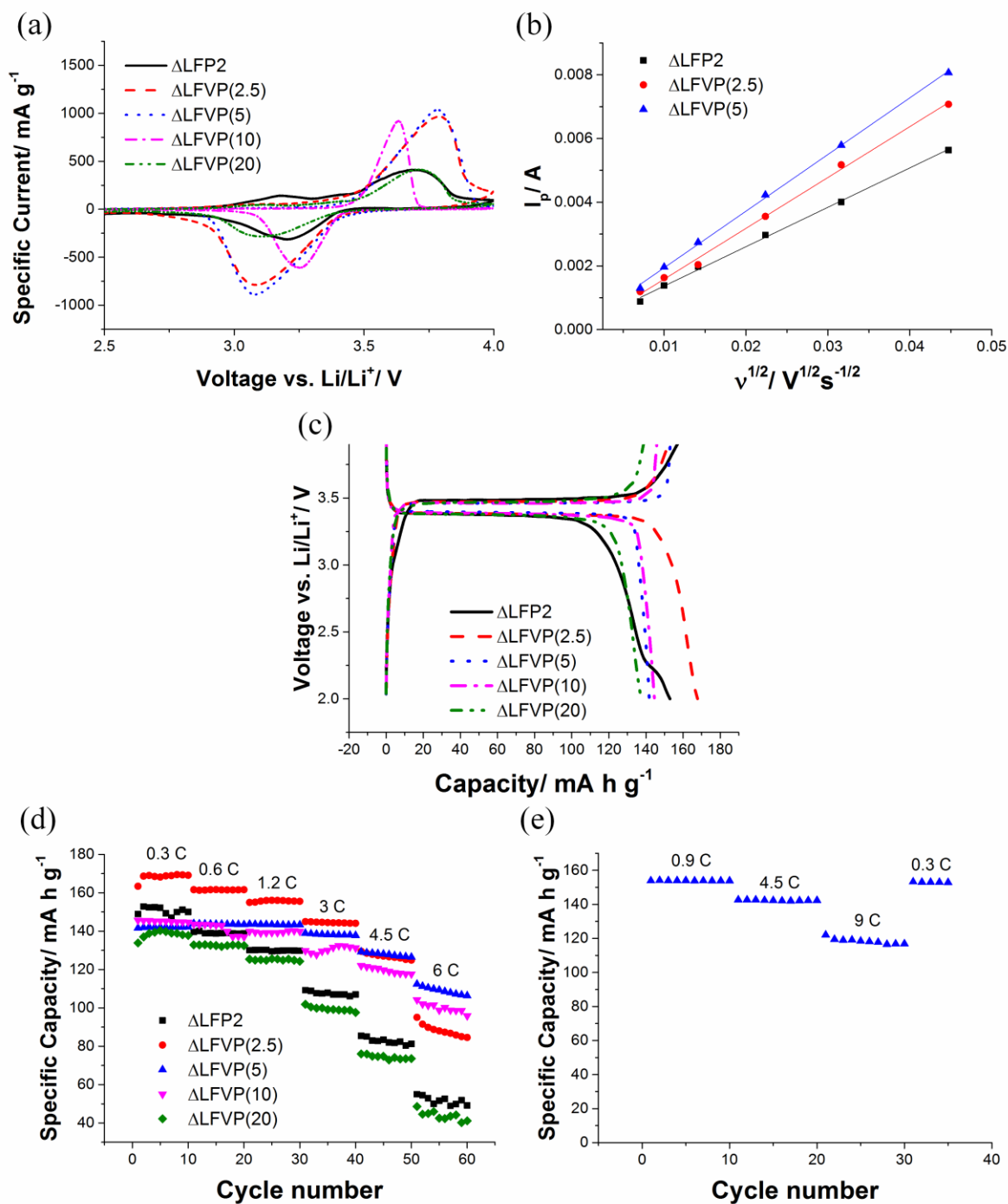
Figure 5. a) Cyclic Voltammety tests (first cycle) at a scan-rate of 0.5 mV s -1 , b) Linear fits of peak current against v^{1/2} for samples \Delta LFP2, \Delta LFVP(2.5) and \Delta LFVP(5), c) Voltage vs. capacity plots of all samples (10 th cycle at 0.3 C), d) Constant current tests at the C-rates shown and e) Further constant current tests of \Delta LFVP(5) at the C-rates shown. The sample \Delta LFVP(5) was consistently shown to be best performing across these tests.
