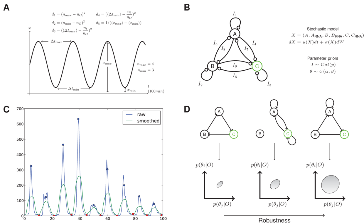
Figure 1. Outline of the method. (A) The objective behavior is specified through a set of summary statistics and distances on the summaries (see Materials and Methods for a description of the terms). (B) Model space is defined through a fully connected network. A mapping from the graphical network to a stochastic model is defined together with a prior on the parameters and priors on the allowed networks. (C) Simple signal processing methods are used to extract features from model simulations. The blue and red circles indicate identified maxima and minima, respectively. (D) As the algorithm proceeds the (multidimensional) objective is achieved via small increments using sequential Monte Carlo. The final output of the algorithm is a set of models that satisfy the objective and maximize robustness.
