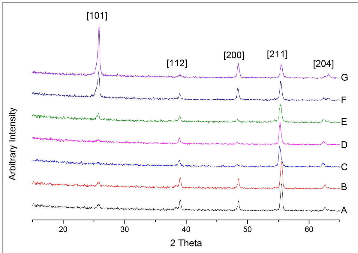
Figure 3: A graph comparing the XRD pattern from all samples A – G grown at 500 °C by combinatorial AACVD. All samples are seen to exhibit crystal structure concordant with anatase \text{TiO}_2 . A change in the prevalence of peaks and shifting is evident across the samples. A change in intensity is particularly acute in the [101] and [200] planes. The [112] and [211] planes exhibit little change in intensity, however the [211] exhibits a shift in its 2\theta value as focus moves from left to right across the width of the film.
