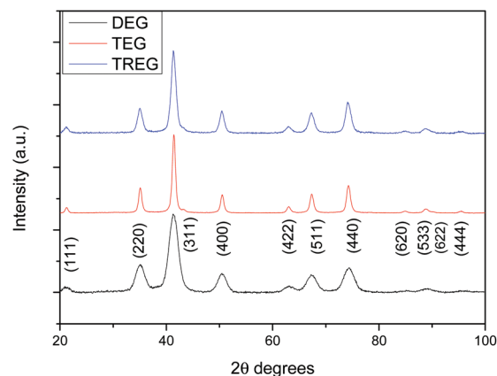
Fig. 5 XRD pattern of IONPs synthesized in different polyol solvents (DEG, TREG and TEG). Peaks have been indexed according to the reference pattern for magnetite (pdf ref. 01-088-0315). Diffraction patterns have been normalised and offset along the y-axis for better comparison.
