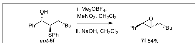
Scheme 5 Conversion of a \beta -hydroxysulfide into an enantioenriched 1,2-disubstituted epoxide
