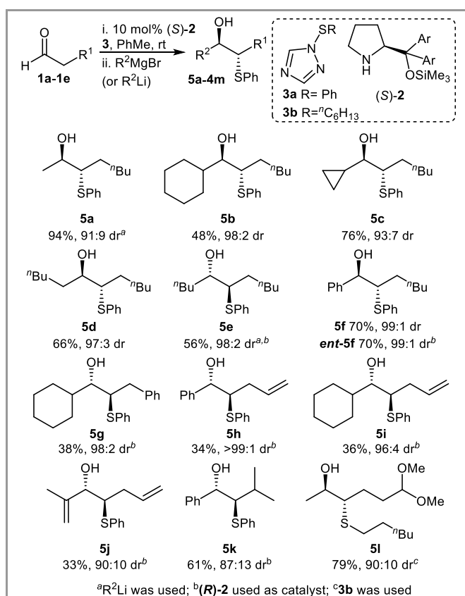
Scheme 3 Synthesis of \beta -hydroxysulfides via organocatalytic sulfenylation of aldehydes followed by organometallic addition.
