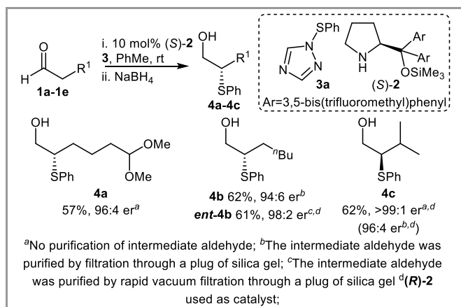
Scheme 2 Asymmetric organocatalytic \alpha -phenylsulfenylation of aldehydes using the Jorgensen-Hayashi catalyst.
