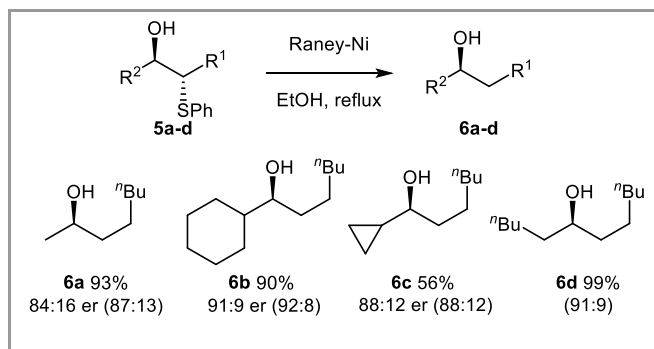
Scheme 4 Desulfurisation of \beta -hydroxysulfides to give enantioenriched secondary alcohols. Enantiomeric ratios were determined via formation of the Mosher's esters; 11 calculated enantiomeric ratios are shown in parentheses. 15
