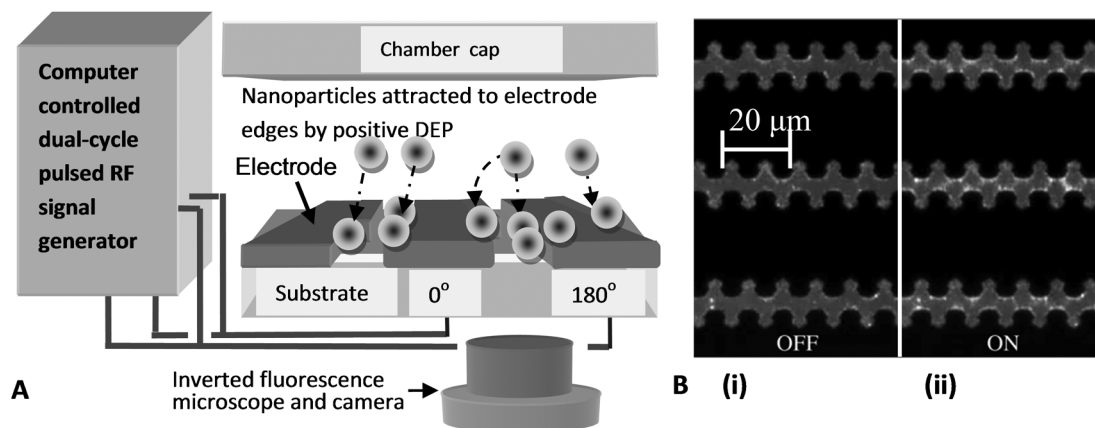
Figure 1. (A) Schematic of a typical experimental arrangement showing nanoparticles being attracted by pDEP onto microfabricated planar castellated electrodes, connected to a signal supply, as shown. The experiment is imaged using an inverted fluorescence microscope (not to scale, see text for details). (B) Typical partial-frame images of fluorescent nanoparticles with pDEP (i) off and (ii) on . The dark regions are the castellated electrodes. During the “on” state fluorescently labelled nanoparticles collect at the electrode tips as an AC signal is applied.
