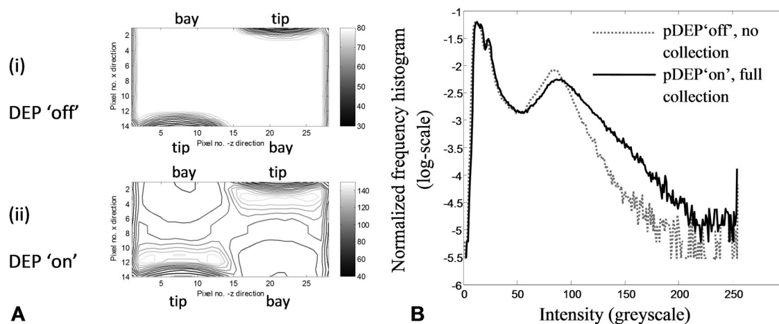
Figure 3. (A) Intensity contours (grayscale units) for the rectangular region of interest representing the fluorescence intensity measured over the interelectrode gap (castellated electrode tips and bay regions as labelled). (i) DEP “off” —the dark contours indicate the electrode edges and the lighter areas are due to scattered light that is uniformly distributed, as shown by the absence of contours. (ii) DEP “on” —light gray contours, with grayscale values well above scattered light, show pDEP-driven nanoparticle collections near the electrode tips and across the interelectrode gap. On the other hand, nanoparticle depletion is indicated by darker contours associated with the bay regions. (B) Statistical filtering considers the pixel intensity distribution (normalized frequency histogram) for the entire frame. The gray dotted curve shows the distribution for the pDEP “off” state; the black full curve shows the distribution for the pDEP “on” state. By choosing appropriate statistics sensitive to the distribution spread or SD, the different off–on states can be detected without needing user input data.
