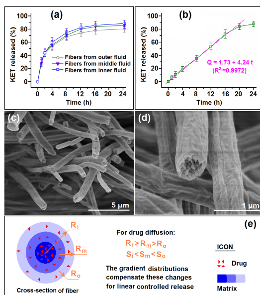
Figure 7. (a) and (b) In vitro dissolution test results of the monolithic nanofibers and the tri-layer nanofibers, (c) and (d) FESEM images of the tri-layer nanofibers after release of all the KET loading, and (e) a diagram explaining how the gradient drug distribution can yield a linear release profile.
