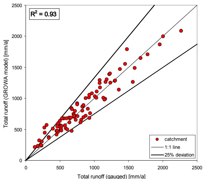
Figure 5-3: Comparison of gauged and modelled total runoff in Slovenia (95 catchments).
