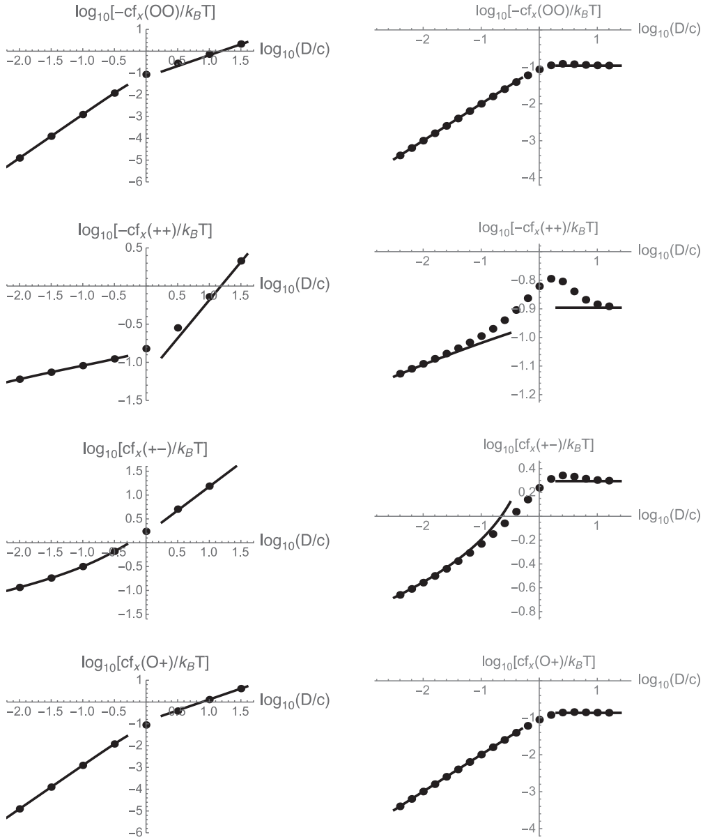
FIG. 5. Component f_x of the force exerted on needle I by needle II for needles with separation c = z_1 - z_2 in the symmetric-parallel configuration (B) in Fig. 3. The results in the left and right columns are for needles of the same length D_I = D_{II} = D and for needles with different lengths, D_I = D and D_{II} = c , respectively. The points indicate the numerical predictions of our exact approach, and the curves show the asymptotic forms derived in the text for large and small D/c . The force component f_y and the torque vanish due to symmetry. For more details, see Sec. V.
