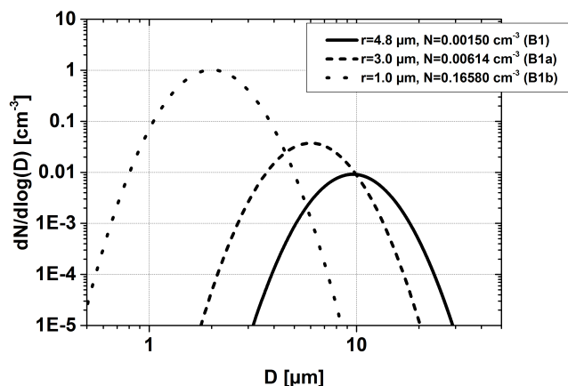
Figure B1. Size distributions used for sensitivity simulations discussed in Appendix B. The total volume of condensed \beta -NAT is constant (corresponding to 8.4 ppbv of gas-phase equivalent \text{HNO}_3 ) and the mode width is 1.35 in all cases. For the binned size distribution used in the AR = 0.1 scenario with r = 1.0 , the particle number density had to be scaled to 0.17342\text{ cm}^{-3} to match 8.4 ppbv of gas-phase equivalent \text{HNO}_3 .
