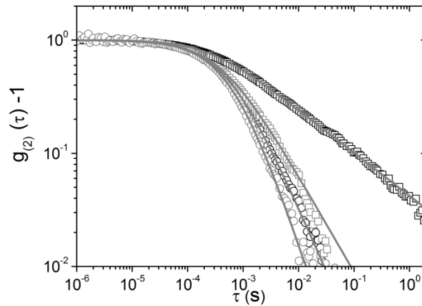
Figure 2: Intensity autocorrelation functions at \theta=90^\circ from xanthan solutions of 0.03 ( \circ ), 0.3 ( \circ ), 0.6 ( \square ) and 1.4 ( \square ) mg/ml (with 0.03M NaCl). Lines are fits with equation (3).
