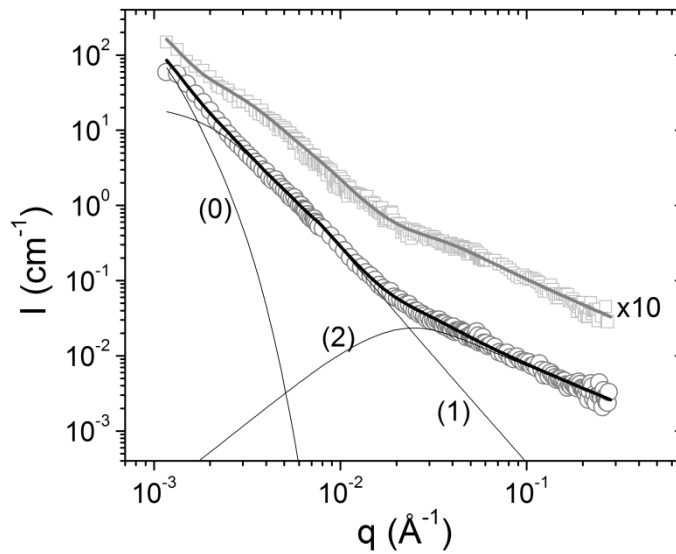
Figure 8: SANS profiles from xanthan solutions at 8 (○) and 10 (□) mg/ml for extended q range. Continuous lines are fitting curves. The separate contributions of equation 5 are shown for 8 mg/ml.
