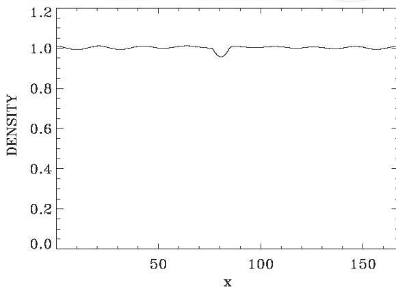
Fig. 24. Electron density profile at t=2980 .
