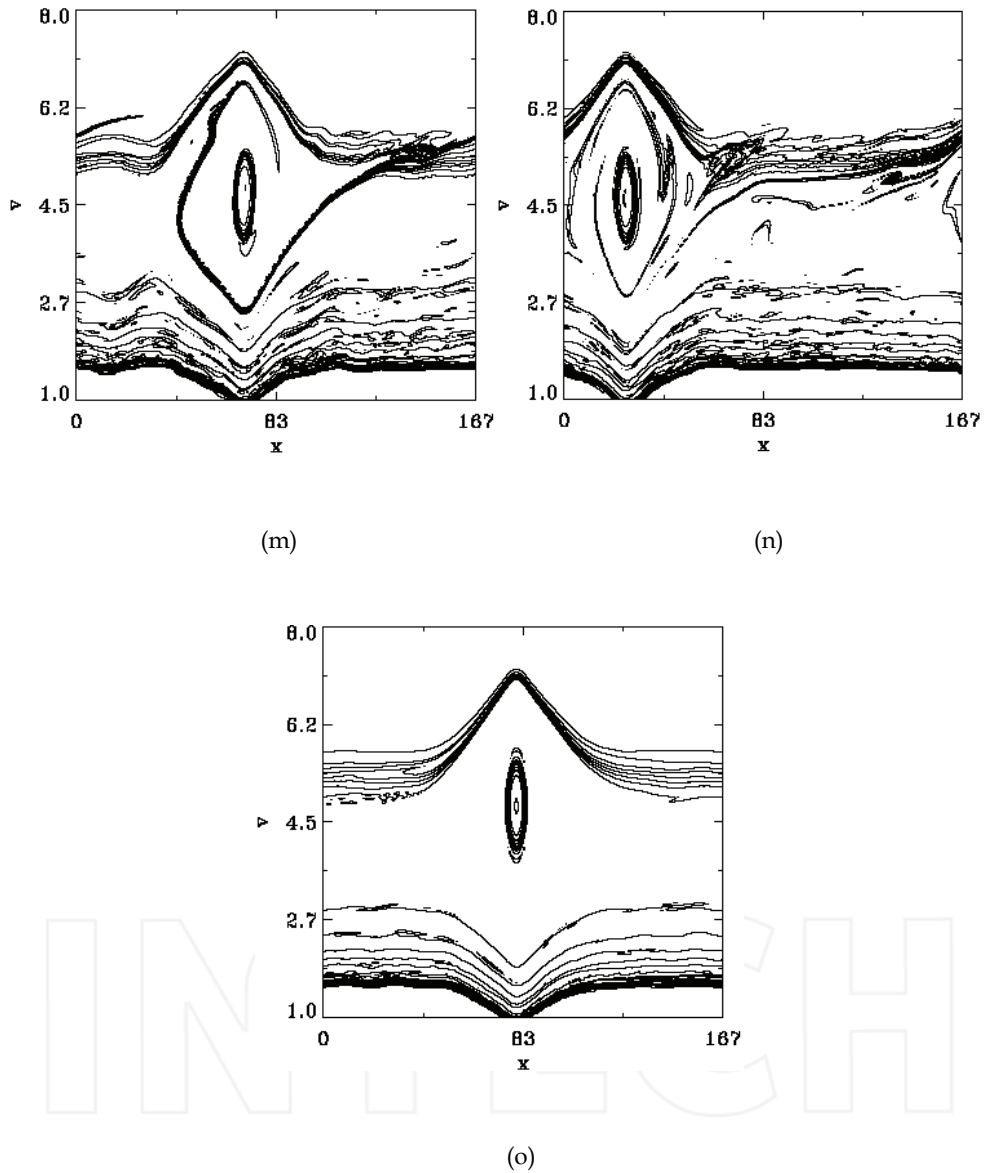
Fig. 7. (m) Contour plot of the distribution function, t=2000 , (n) Contour plot of the distribution function, t=2200 , (o) Contour plot of the distribution function, t=2980 .
