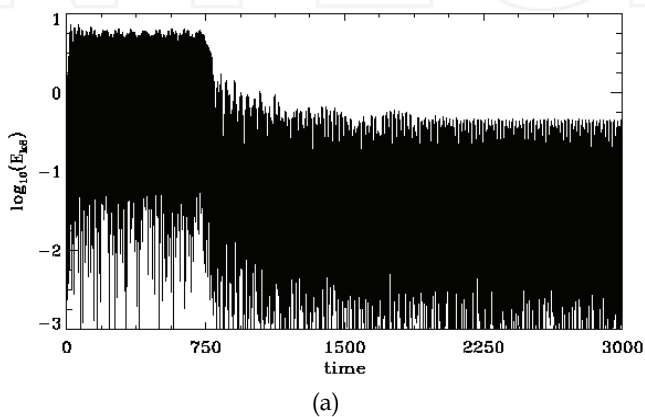
Fig. 18. (a) Time evolution of the Fourier mode with k=0.2625 , (b) Spectrum of the Fourier mode k=0.2625
