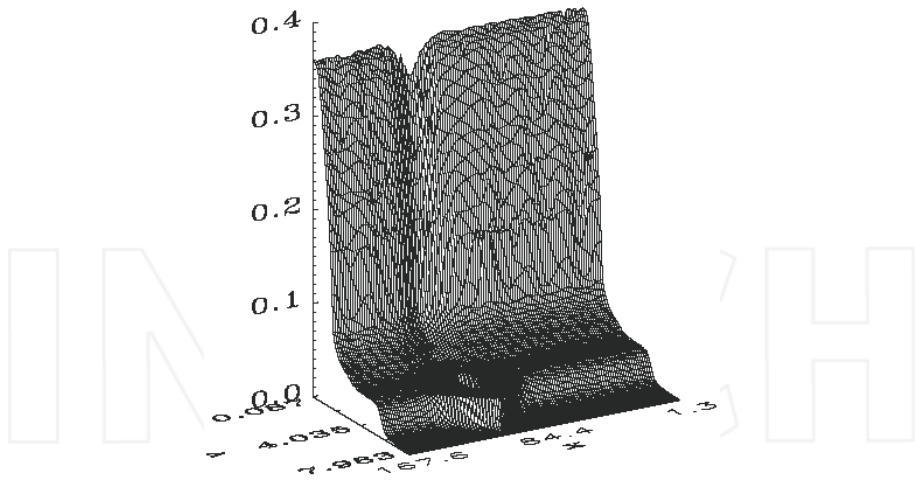
Fig. 28. Same as Fig.(27o), 3D plot at t = 3000
