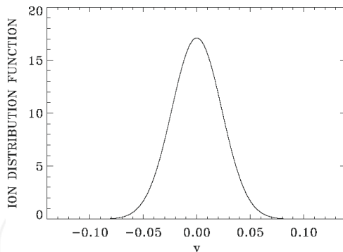
Fig. 10. Ion distribution function at t = 2980
