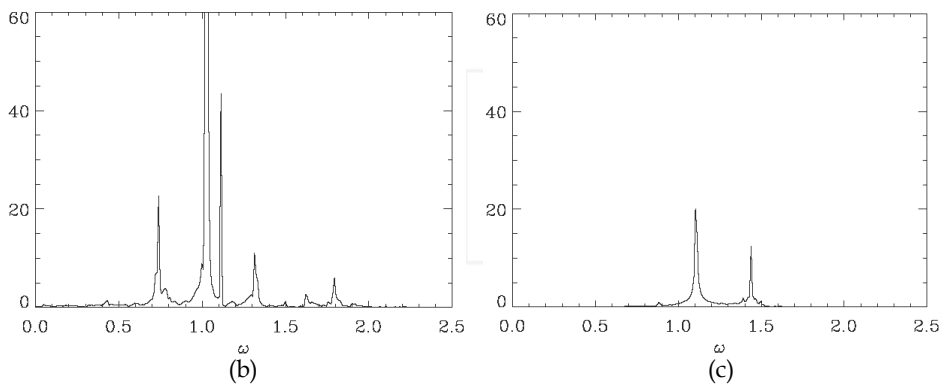
Fig. 19. (a) Time evolution of the Fourier mode with k=0.3 , (b) Spectrum of the Fourier mode k=0.3 (from t=100 to t=755.36 ), (c) Spectrum of the Fourier mode k=0.3 (from t=2344 to t=3000 )
