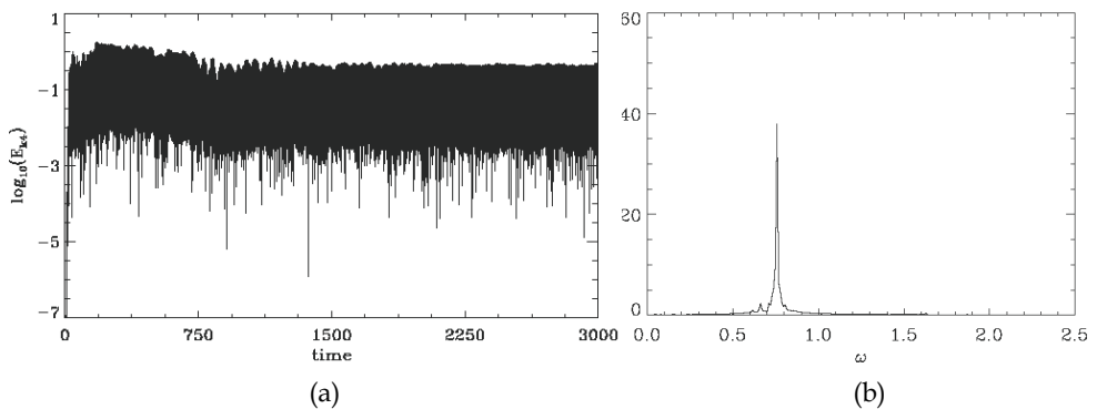
Fig. 35. (a) Time evolution of the Fourier mode k=0.15 (b) Spectrum of the Fourier mode k=0.15
