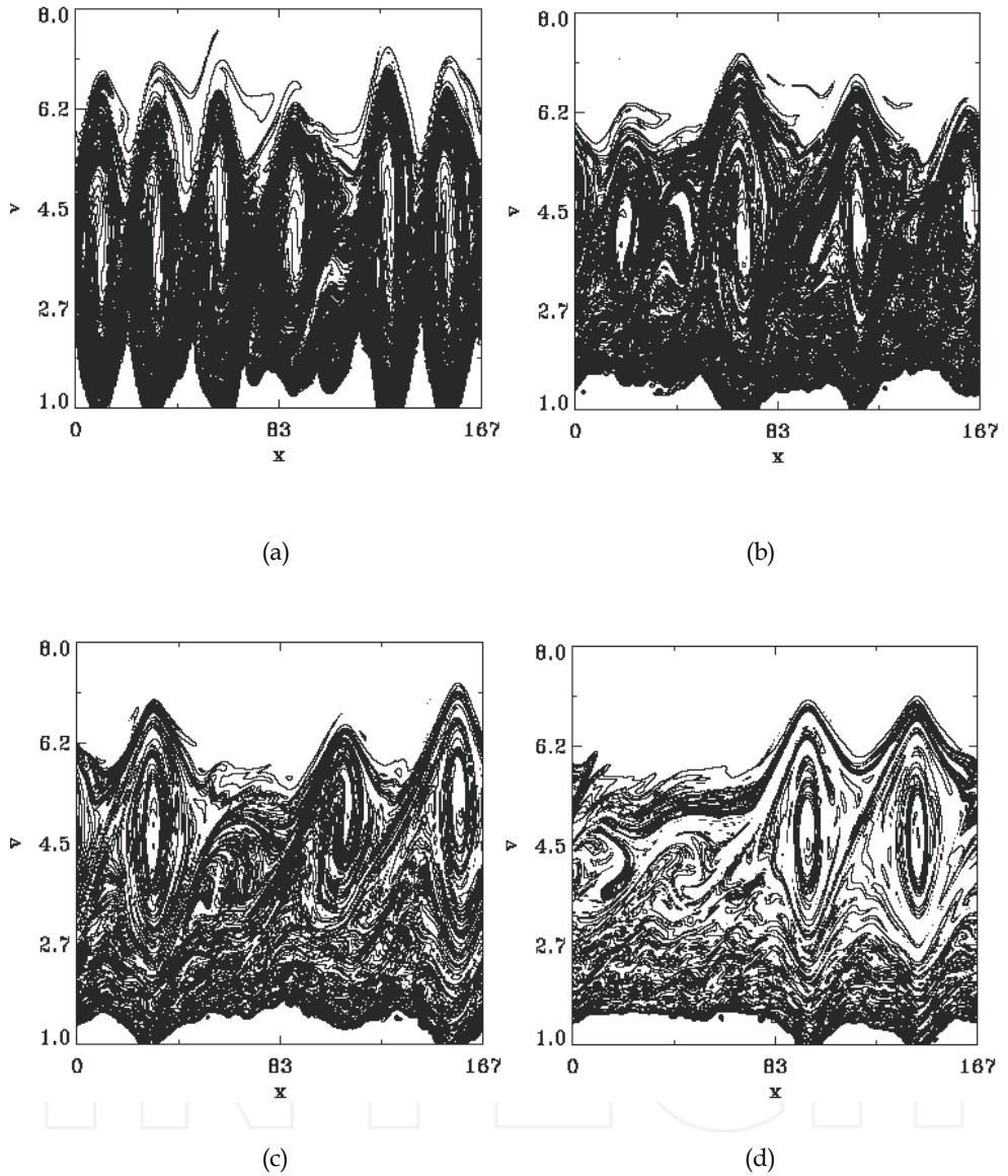
Fig. 27. (a) Contour plot of the distribution function, t = 60 (b) Contour plot of the distribution function, t = 200 (c) Contour plot of the distribution function, t = 400 (d) Contour plot of the distribution function, t = 600
