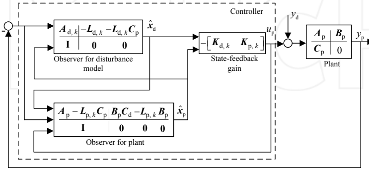
Figure 6. Detailed illustration of observer structure
