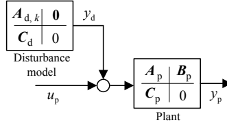
Figure 4. System model for the disturbance observer approach
