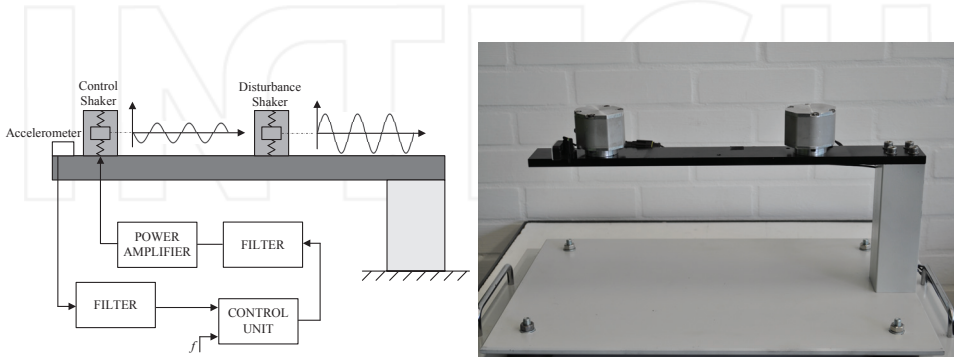
Figure 15. Schematic representation (left) and photograph (right) of the AVC system
