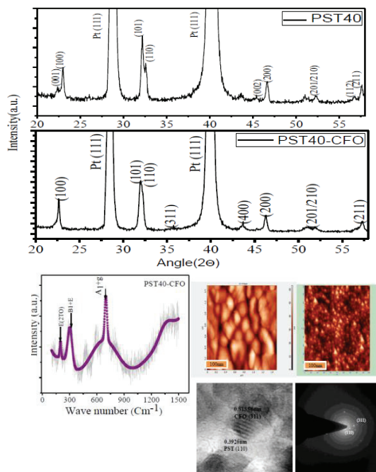
FIGURE 1. (a) XRD pattern of PST and PST40-CFO (b) Raman spectra, AFM and TEM images of CFO, PST40-CFO nanostructure.
