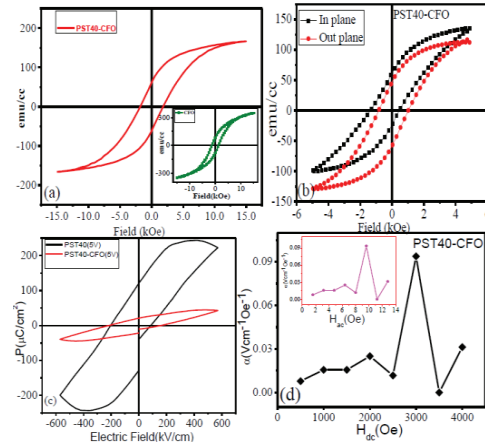
FIGURE 2. (a) MH (b) in-plane and out plane hysteresis curves (c) PE and (d) ME of Pb 0.60 Sr 0.40 TiO 3 -CoFe 2 O 4 nanostructured bilayer thin
