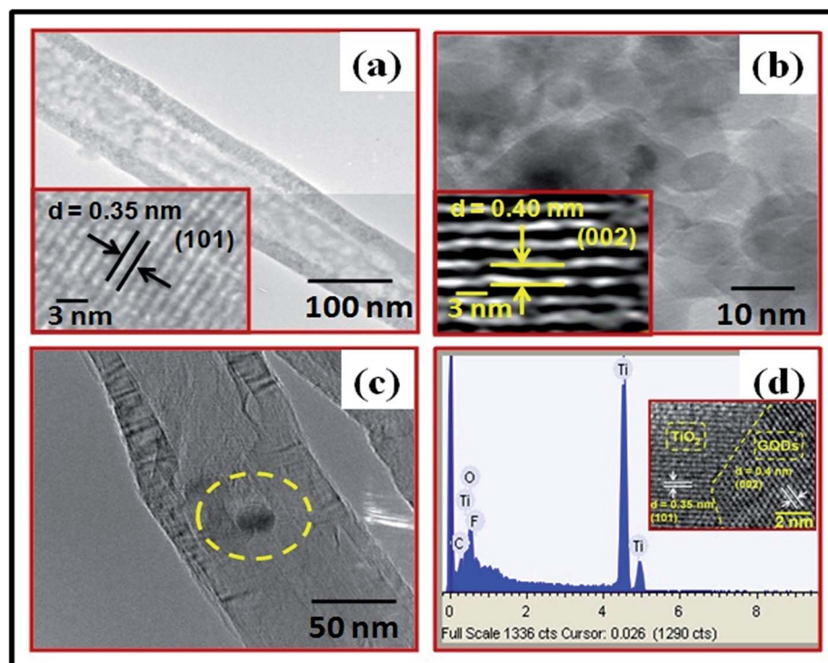
Fig. 7 (a) TEM image of an isolated annealed \text{TiO}_2 nanotube; inset shows the HRTEM image of (a), (b) TEM image of GQDs; inset shows the HRTEM image of (b), (c) TEM image of GQDs infilled isolated \text{TiO}_2 nanotube; yellow circle represents the GQD particle and (d) EDAX spectrum of GQDs infilled \text{TiO}_2 3D NTAs; inset shows the HRTEM image of GQDs infilled \text{TiO}_2 NTAs where yellow mark line clearly reveals the separate lattice of the GQDs and \text{TiO}_2 .
