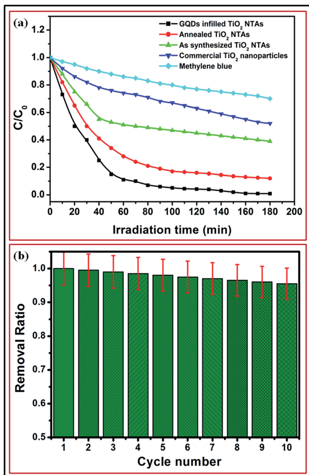
Fig. 10 (a) Comparative studies on photocatalytic activity versus UV irradiation time for pristine methylene blue, commercial TiO 2 (size ~50 nm), as synthesized TiO 2 nanotubes, annealed TiO 2 nanotubes and GQD infilled TiO 2 NTAs and (b) cycle stability data of the GQD infilled TiO 2 NTAs.
