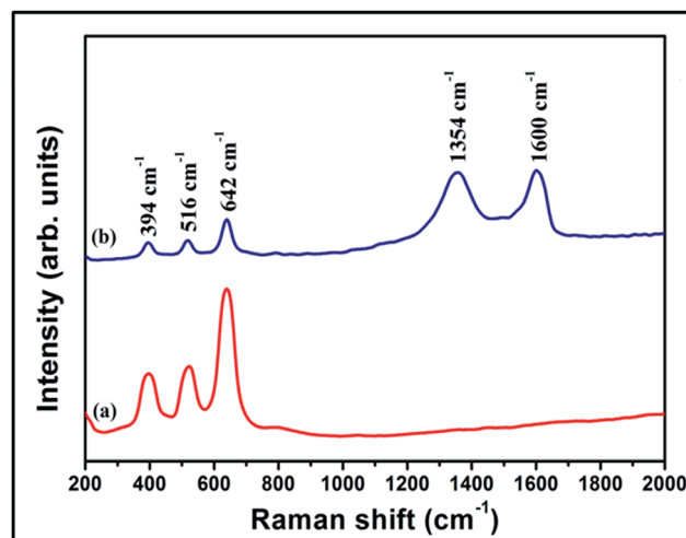
Fig. 4 Raman spectra of (a) annealed \text{TiO}_2 3D NTAs and (b) GQDs infiltrated \text{TiO}_2 3D NTAs.
