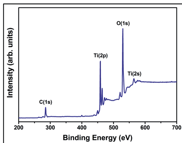
Fig. 5 XPS spectrum of GQDs infiltrated \text{TiO}_2 3D NTAs.
