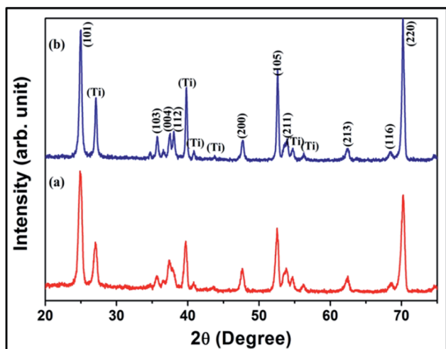
Fig. 3 The XRD patterns of (a) annealed \text{TiO}_2 3D NTAs and (b) GQDs infiltrated \text{TiO}_2 3D NTAs.
