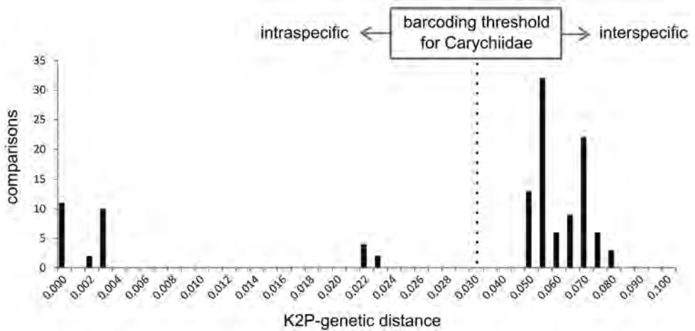
Figure 6. Overview of pairwise genetic distance measurements.
