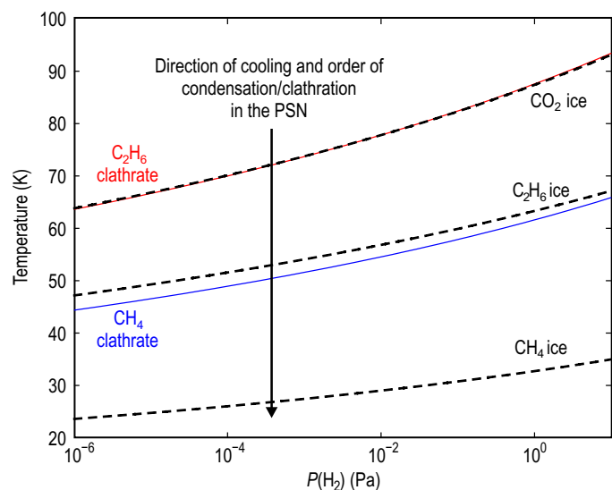
Fig. 1. Equilibrium curves of clathrates and condensation in the PSN. Equilibrium curves of C 2 H 6 (red) and CH 4 (blue) clathrates are shown with respect to the equilibrium curves of C 2 H 6 , CH 4 , and CO 2 ices (black dashed lines) as a function of total nebular pressure. The arrow indicates the direction of cooling in the PSN. Above the clathrate stability/condensation curve, a volatile species exists in the gas phase. Below the clathrate stability/condensation curve, a volatile species may form clathrates or pure condensates. The gas-phase mole fractions relative to H 2 were derived from the cometary X/H 2 O ratios (14) and solar system elemental abundances of O and H (40, 41).
