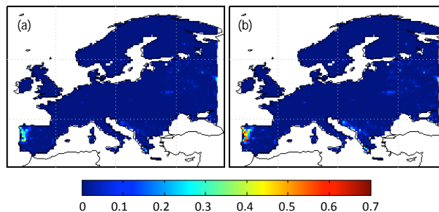
Figure 6. Wildfire \text{PM}_{2.5} emissions during peak fire season displayed on linear scale, in \text{g (m}^2 \text{ month)}^{-1} : (a) current and (b) 2090.
