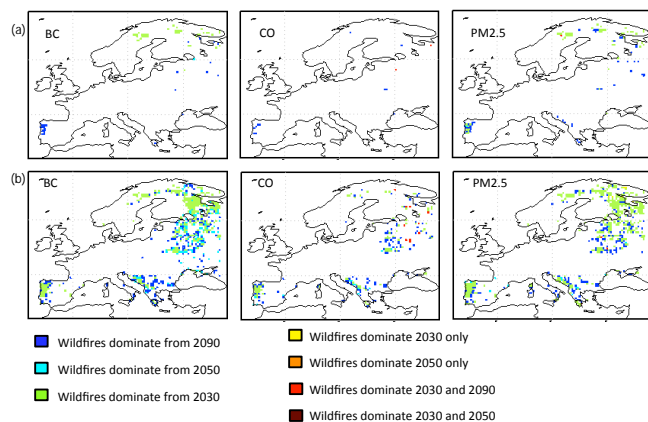
Figure 5. Areas where wildfire emissions exceed anthropogenic emissions in 2030, 2050 or 2090 on annual basis (a) or during peak fire season (b) (month of maximum wildfire emissions varying by grid cell), assuming RCP8.5 climate, SSP5 population and maximum feasible reduction anthropogenic emissions.
